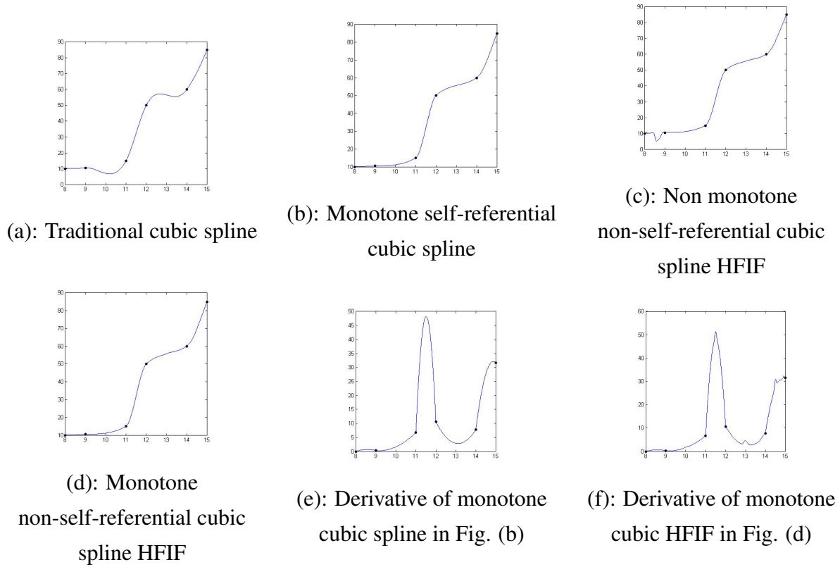
Figure 3: Cubic spline hidden variable fractal interpolation functions (HFIFs) (the interpolating data points are given by the circles and the relevant hidden variable fractal interpolants by the solid lines).
