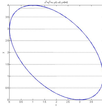
Figure 1: Fritsch-Carlson monotone region.
