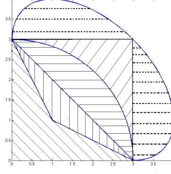
Figure 2: Fritsch-Carlson subregions. Diagonal hatching (- slope): \Omega_4 ; Vertical hatching: \Omega_3 - \Omega_4 ; Horizontal hatching: \Omega_2 - \Omega_3 ; Diagonal hatching (+ slope): \Omega_1 - \Omega_2 ; Dotted: \mathcal{M} - \Omega_1 .
