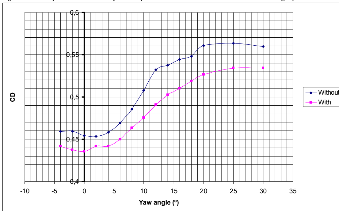
Fig. 6. Plot of yaw angle versus Cd for the Honda Civic Wind Tunnel Tests. Bibliographical source: "Lockheed Georgia Low Speed Wind Tunnel Honda Civic Hatchback Air tab(R) Modification Results"13
