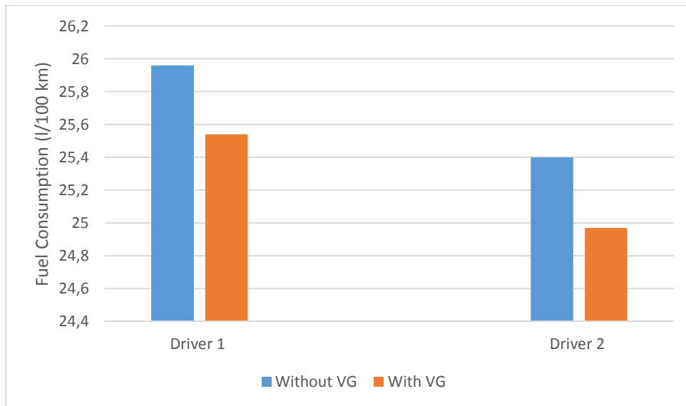
Fig. 5. MIRA experimental results for heavy vehicles with and without Air TAB Bibliographical source: IRTE6
