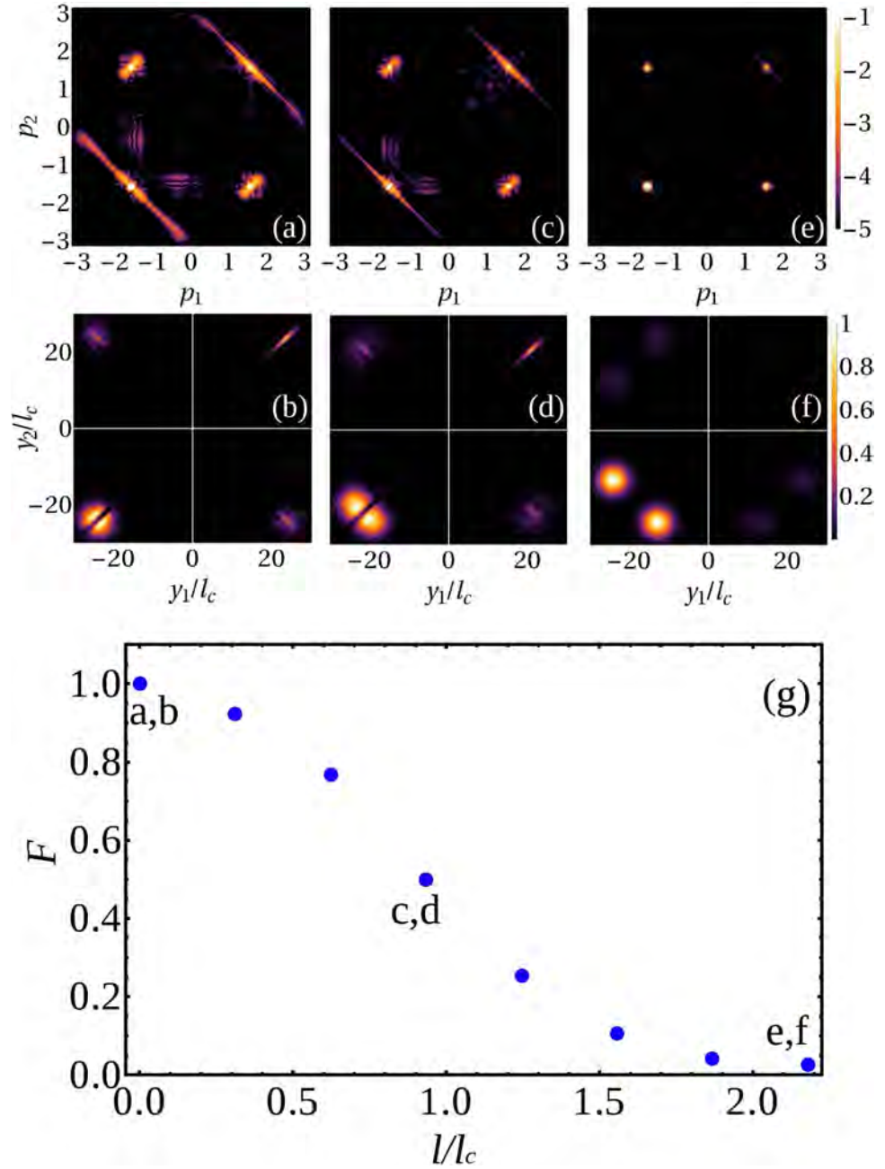
Figure 3. Output wave function in momentum/position space, (a)/(b), (c)/(d), and (e)/(f) for several values of the distance between the input photons and (g) fluorescence F for the two-photon output state as a function of the distance l between the two input wave packets. The values of the distances of the panels (a)–(f) are indicated in panel (g). We choose g = 0.3 . The values for the other parameters coincide with those of figure 2. Both incoming photons are on resonance with the qubit, \omega_k = \Delta . The distance l is in units of l_c \simeq 1.719\sigma , with l_c such that we can resolve the incident packets if and only if l > l_c .
