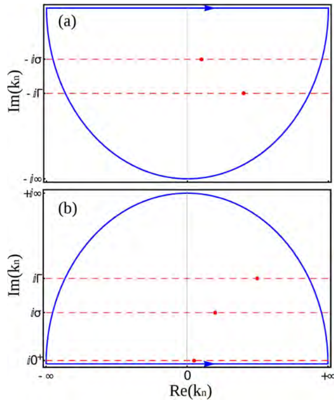
Figure G1. (a) Lower and (b) upper contour for integrating equation (33). We show the poles coming from the Lorentzian, \pm i\sigma , those coming from one of the transmission amplitudes or from C , \pm i\Gamma , and those with vanishing imaginary part. The real parts are arbitrary.
