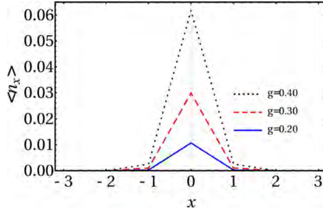
Figure 2. Number of excitations in position space of the minimum-energy state of (25) for \epsilon = 1 , J = 1/\pi , and \Delta = 1 , varying g . The coordinate x is dimensionless, since we are working in units such that the lattice spacing b is 1.
