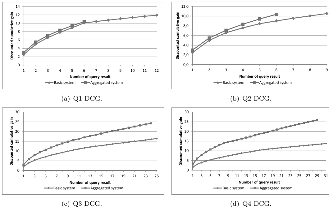
Figure 6. Detailed DCG comparison of the analyzed queries.
