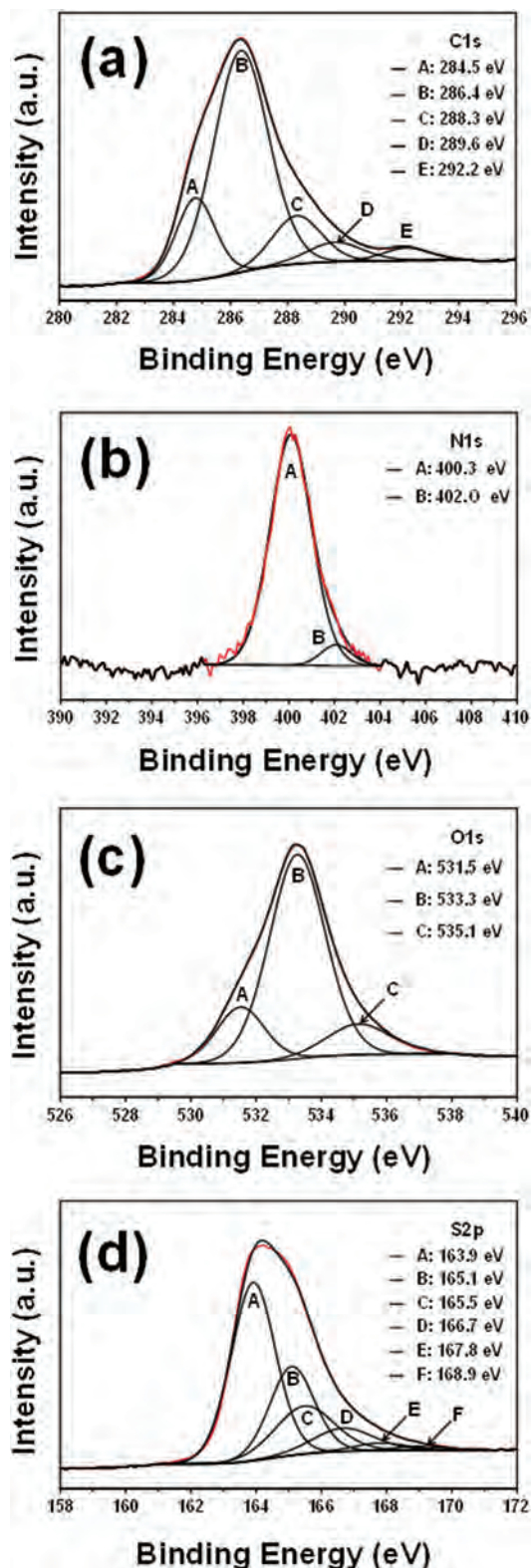
Fig. 4 High-resolution XPS spectra for PEDOT-RG E D/B: C 1s (a), N 1s (b), O 1s (c) and S 2p (d) regions. Peaks from deconvolution are also displayed. The red line corresponds to the experimental profile while the black line is the sum of the deconvoluted peaks.
