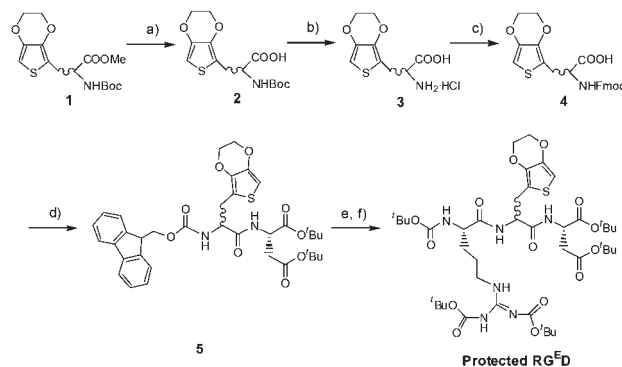
Fig. 1 Reagents and conditions for the synthesis of protected RG E D: (a) KOH 2 N/MeOH, rt 2 h, 99%; (b) HCl (3N)/AcOEt, rt 30 min, 100%; (c) FmocOsu, K 2 CO 3 , CH 3 CN/H 2 O 3/1, 80%; (d) HOBt, EDC-HCl, NMM, H-L-Asp(O t Bu)-O t Bu, CH 2 Cl 2 , 0 °C 30 min, rt 24 h, 95%; (e) DEA, CH 2 Cl 2 , rt 4 h, 100%; (f) HOBt, EDC-HCl, NMM, Boc-L-Arg(Boc) 2 -OH, CH 2 Cl 2 , 0 °C 30 min, rt 24 h, 90%.
