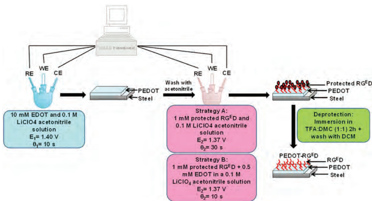
Fig. 2 Scheme displaying the two synthetic strategies (A and B) used to prepare PEDOT-RG ED . Each strategy involved a three-step process, even though A and B only differ in the conditions used for the intermediate step. RE, WE and CE refer to the reference electrode, working electrode and counter electrode, respectively.
