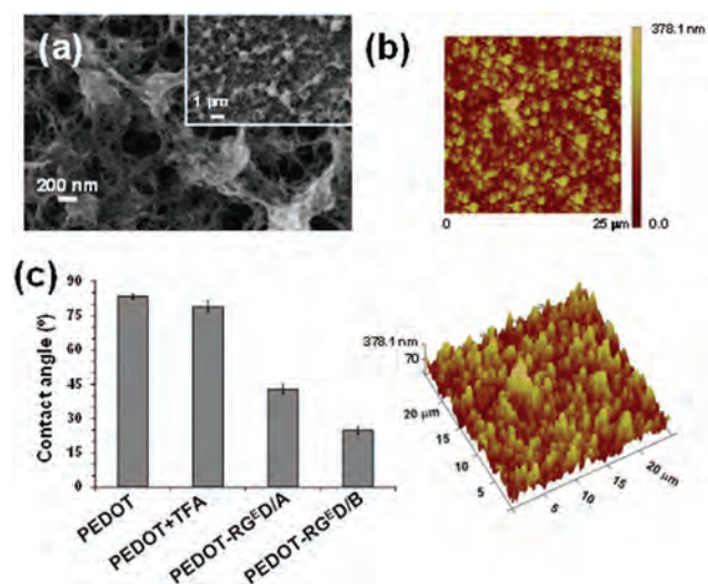
Fig. 5 (a) SEM micrographs, high and low (inset) magnifications, and (b) 2D and 3D topographic images of PEDOT-RG E D/B. (c) Contact angles of water (average and standard deviation of 14 independent measures) for as prepared PEDOT, PEDOT treated with 1 : 1 TFA : DCM for 2 hours and, subsequently, washed with DCM (PEDOT + TFA), emulating the step used to eliminate the protection of peptide fragments in PEDOT-(protected RG E D) systems, and the two prepared conjugates.
