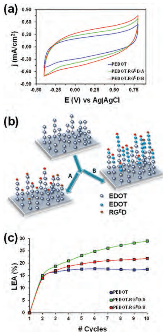
Fig. 6 (a) Control voltammograms of PEDOT, PEDOT-RG E D/A and PEDOT-RG E D/B in PBS. Initial and final potentials, -0.40 V; reversal potential, 0.80 V; scan rate, 50 mV s -1 . (b) Scheme reflecting surface structural differences between PEDOT-RG E D/A and PEDOT-RG E D/B conjugates. (c) Loss of electroactivity (LEA) against the number of consecutive oxidation and reduction cycles in 0.1 M PBS for PEDOT, PEDOT-RG E D/A and PEDOT-RG E D/B.
