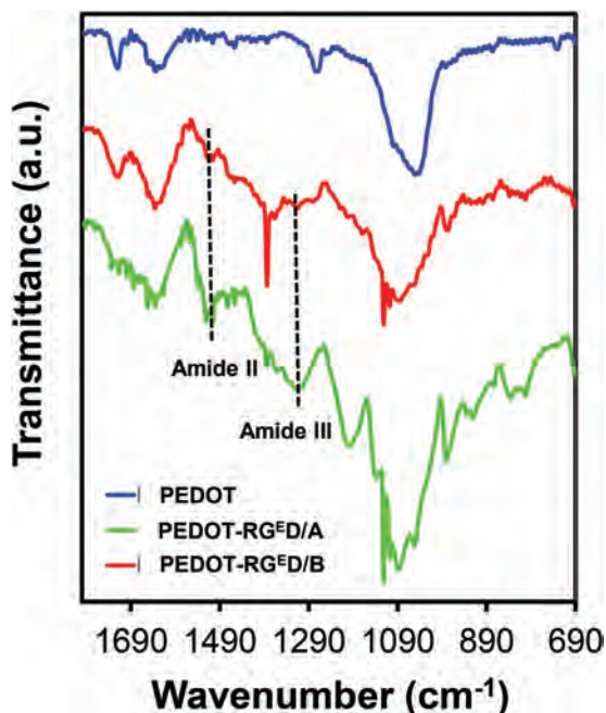
Fig. 3 FTIR spectra of PEDOT, PEDOT-RG E D/A and PEDOT-RG E D/B.
