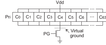
Fig. 3. Implementation of the NBTI-aware power-gating technique.
