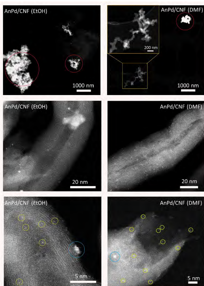
Fig. 10 HAADF-STEM images of the catalysts at different magnifications showing the presence of Pd sub-nanometric particles (yellow circles) and large Pd aggregates (red circles).
