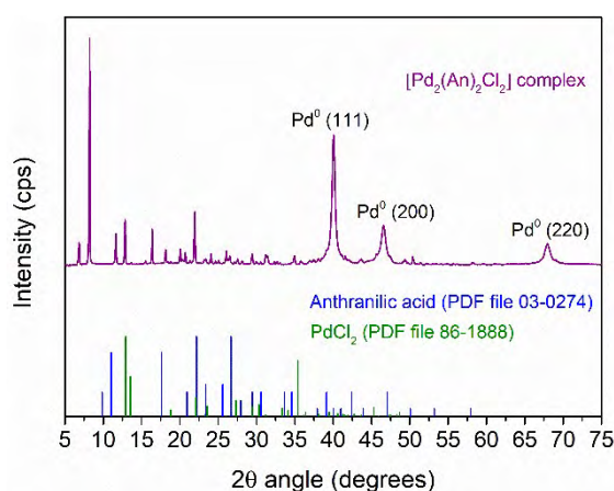
Fig. 5 Powder XRD pattern of the synthesized [Pd 2 (An) 2 Cl 2 ] complex.
