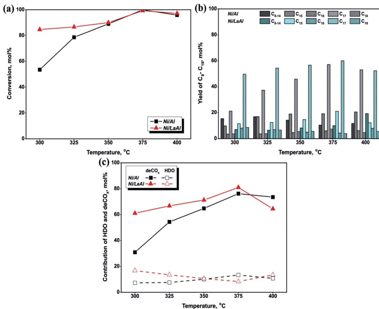
Fig. 6 Effect of temperature on: (a) palm oil conversion, (b) paraffin yield, and (c) % contribution of HDO and deCO x for the Ni/Al and Ni/LaAl catalysts. Reaction conditions: T = 300\text{--}400 °C, P = 30 bar, LHSV = 1.2 h -1 , H_2/oil = 1000 cm 3 (cm 3 ) -1 .
