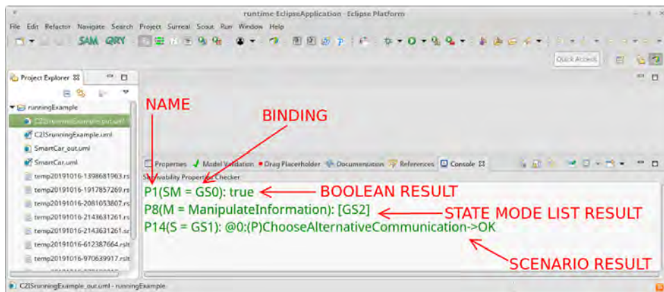
Fig. 8. The running example – assessment report.
