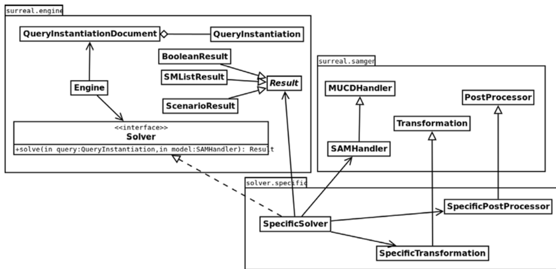
Fig. 9. Class diagram for extending solvers in the surreal framework.
