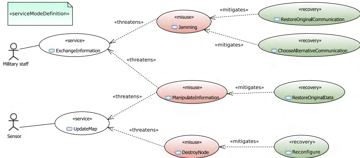
Fig. 3. MUCD of the running example annotated with the survivability profile.
