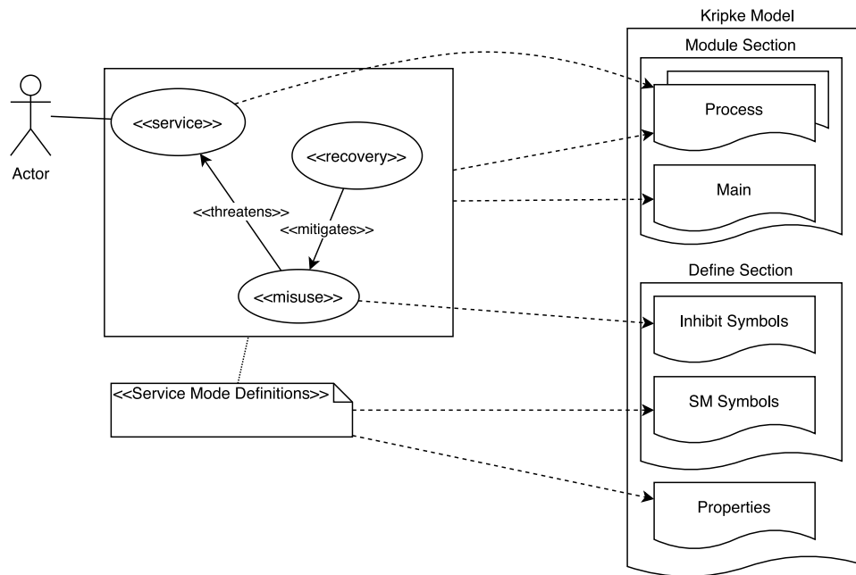
Fig. 5. MUCD-to-Kripke: overview.
