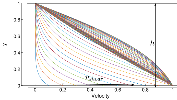
Fig. 7. Evolution of the velocity profile at the startup of shear flow in an Oldroyd-B fluid. The different lines represent the velocity profile at different time instants. Note the overshoot in the profile, that tends to the linear profile, typical of a Couette flow, for sufficiently large time. Velocity profile at every t = 0.01 seconds ( t \in (0, 1.5] ). Velocity is imposed at the bottom plate, with h = 1.0 and v_{\text{shear}} = 1.0 .
