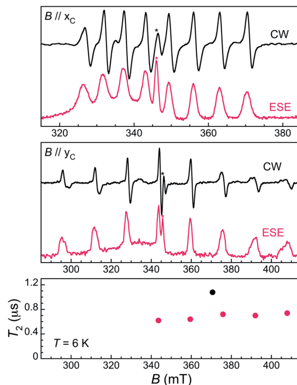
Fig. 4 Top: X-band CW (RT, black lines) and 2p-ESE-detected (6 K, \tau = 200 \text{ ns} , red lines) EPR spectra of 1_{3\%}^{\text{VO}} with the field along the x_C (top) and y_C (middle) crystal axes. Bottom: coherence time T_2 for 1_{3\%}^{\text{VO}} with the field along the x_C (black symbols) and y_C (red symbols) axes of the crystal. Stars indicate an isotropic signal at g = 2.01 ascribed to a Ti(III) impurity. A broad signal covering the 290–350 mT field range arises from Cu(II) ions on the surface of the cavity.
