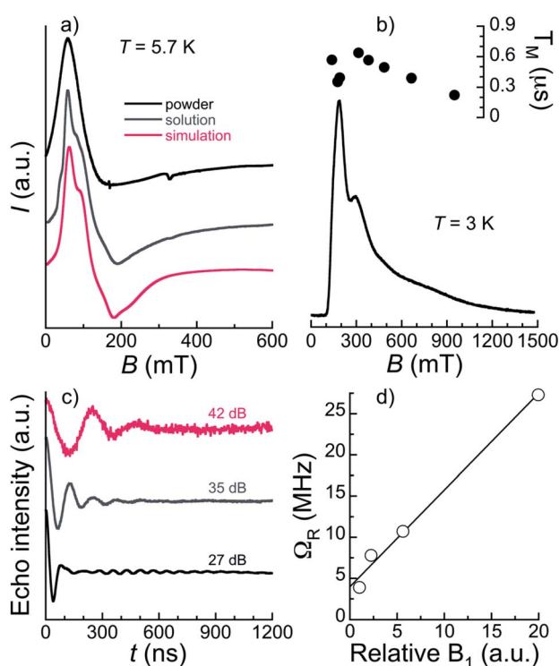
Fig. 6 (a) Comparison of the experimental continuous-wave X-band EPR spectra for bulk polycrystalline 1 (black line) and a frozen solution (5 mM) of 1 at 5.7 K. The red line is a simulation of the latter with parameters g_{Er} = 11.5 ; 5; 1 (as previously measured for ErLaEr) and g_{Pr} = 3.4 . (b) Echo-detected field-swept (EDFS) X-band (ca. 9.70 GHz) EPR spectrum of a frozen solution (2.5 mM) of 1 at 3 K, measured using a Hahn echo sequence with \pi = 32 ns and \tau = 130 ns, together with the values of phase memory times, T_M , derived at various applied fields. (c) Nutation data at three mw attenuations and 330 mT revealing Rabi oscillations for a frozen solution (2.5 mM) of 1 at 3 K. (d) B_1 dependence of the Rabi frequency. The solid line is a guide to the eye, emphasizing the linear dependence expected for qubits.
