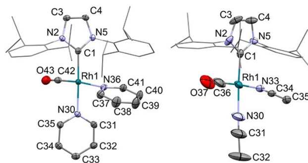
Figure 2. ORTEP view of [\text{Rh}(\text{CO})(\text{IPr})(\text{py})_2]^+ in 4 (left) and [\text{Rh}(\text{CO})(\text{IPr})(\text{CH}_3\text{CN})_2]^+ in 5 (right) with ellipsoids at 50% probability. For clarity hydrogen atoms are omitted and a wireframe style is adopted for the 2,5-(iPr) 2 C 6 H 3 moiety of the IPr ligand. Selected bond lengths (Å) and angles (°) are: 4, Rh1-C42 1.815(3), Rh1-C1 2.010(3), Rh1-N30 2.110(2), Rh1-N36 2.123(2), O43-C42 1.142(4), C1-Rh1-C42 87.98(12), C1-Rh1-N30 177.36(11), C1-Rh1-N36 98.34(10), N30-Rh1-N36 84.22(9); 5, C1-Rh1 1.997(3), C36-Rh1 1.814(5), N30-Rh1 2.055(4), N33-Rh1 2.072(3), C36-O37 1.143(5), C1-Rh1-C36 90.96(16), C1-Rh1-N33 91.96(11), C1-Rh1-N30 177.28(14), N30-Rh1-N33 85.66(13), Rh1-C31-N30 176.4(5), Rh1-C34-N33 170.7(3).
