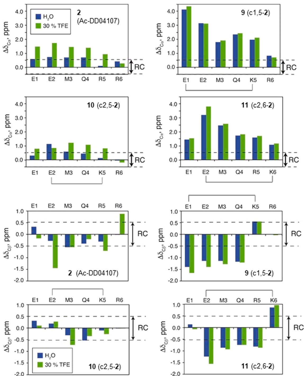
Fig. 5. Bar plots showing the \Delta\delta_{C\alpha} ( \Delta\delta_{C\alpha} = \delta_{C\alpha}^{\text{observed}} - \delta_{C\alpha}^{\text{RC}} , ppm) values and \delta_{C\alpha} ( \delta_{C\alpha} = \delta_{C\alpha}^{\text{observed}} - \delta_{C\alpha}^{\text{RC}} , ppm) as a function of sequence for peptides Ac-DD04107 ( 2 ), 9 , 10 and 11 in aqueous solution (blue bars) and in 30% TFE (green bars) at pH 5.5 and 5 °C. Dashed lines indicate the random coil (RC) ranges, and random coil values were taken from J. Biomol. NMR 1995, 5, 67–81 [32]. (For interpretation of the references to colour in this figure legend, the reader is referred to the web version of this article.)
