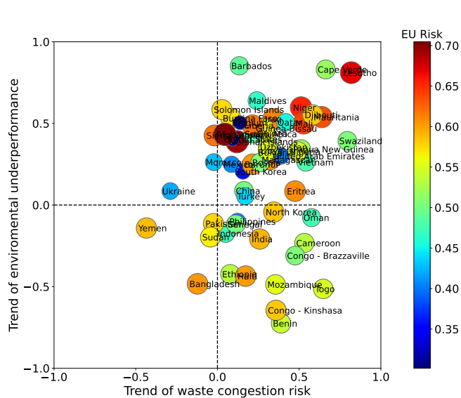
Fig. 4 Temporal trend (period 2001–2019) of the waste congestion risk and of the environmental underperformance risk for some countries at HRIHDW. The trend is measured by the Pearson correlation coefficient between the corresponding variable and the years in the period. Bottom-left quarter identifies the countries with a trend to improve both indices. Top-right quarter identified those countries with a trend to deterioration of both indices. EU Risk stands for Environmental Underperformance Risk.
