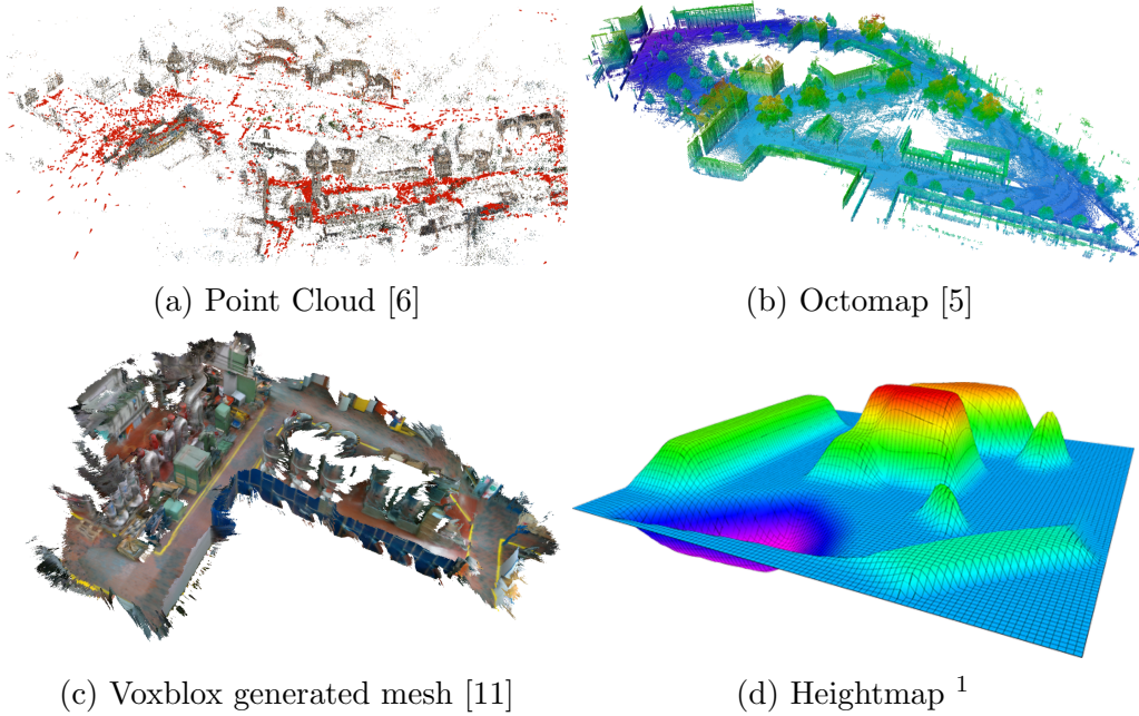
Figure 2.2: Different map representations. Point Clouds (a) are sparse but there are many available processing tools. Octomap (b) is also useful for navigation but it does not account for the quality of represented surfaces. Voxelbox (c) can generate accurate surfaces in real-time and includes implicit information about them which is useful to perform planning based on the surfaces in the map. Despite their simplicity, Heightmaps (d) can be a good solution to scale maps in a computationally efficient way. However, the structural information in the vertical direction is lost.
