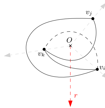
■ Figure 7 If edges v_i v_j and v_j v_k cross r in a c -monotone drawing, then v_i v_k must also cross r .
