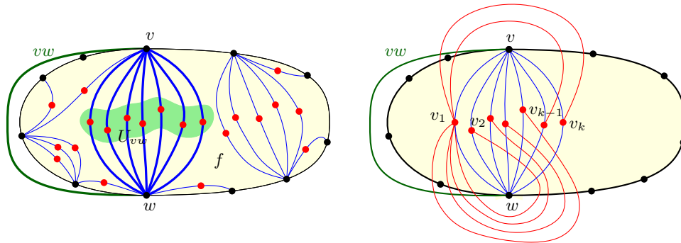
■ Figure 4 The subdrawing D' induced by U_{vw} and the edges in D_{vw} . Left: The set U_{vw} . Right: The edges adjacent to the leftmost vertex, v_1 , are drawn (in red).
