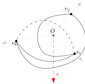
■ Figure 7 If edges v_i v_j and v_j v_k cross r in a c -monotone drawing, then v_i v_k must also cross r .
