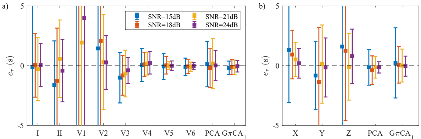
Fig. 5: Estimation error e_\tau (mean \pm standard deviation) in (a) standard leads and (b) orthogonal leads, together with transformed leads obtained by G\pi CA_1 and PCA.
