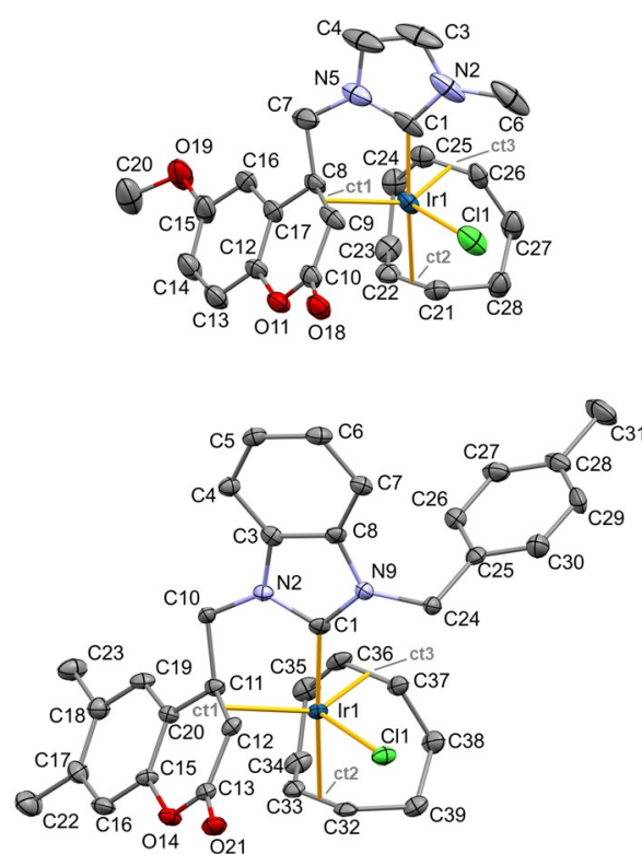
Figure 1. ORTEP view of the crystal structure of 4b (top, 2- \text{CH}_3\text{Cl} ) and 5b (bottom, 1.7- \text{CH}_3\text{Cl} ) with ellipsoids at 50% probability. Hydrogen atoms and lattice chloroform molecules are omitted for clarity. Selected bond lengths (Å) and angles (°) are: 4b , C1–Ir1 2.015(5), C1–Ir1 2.4917(12), Ir1–ct1 2.0548(2), Ir(1)–ct2 2.1796(2), Ir(1)–ct3 2.0055(2), C8–C9 1.441(6), C21–C22 1.373(6), C25–C26 1.442(6), C1–Ir1–Cl1 88.78(15), C1–Ir1–ct1 80.09(14), C1–Ir1–ct2 173.10(12), C1–Ir1–Cl1 108.10(3), ct1–Ir1–ct3 134.522(10), ct3–Ir1–Cl1 115.74(3); ct1, centroid of C8 and C9; ct2, centroid of C21 and C22; ct3, centroid of C25 and C26; 5b , C1–Ir1 2.010(5), Cl1–Ir1 2.4999(12), Ir1–ct1 2.0610(2), Ir1–ct2 2.1744(2), Ir1–ct3 2.0322(2), C11–C12 1.439(6), C32–C33 1.378(7), C36–C37 1.432(7), C1–Ir1–Cl1 87.51(13), C1–Ir1–ct2 175.08(13), C1–Ir1–ct1 80.53(14), C1–Ir1–ct2 102.781(9), ct1–Ir1–ct3 135.518(9), ct3–Ir1–Cl1 115.34(3), ct1–Ir1–Cl1 107.81(3); ct1, centroid of C11 and C12; ct2, centroid of C32 and C33; ct3, centroid of C36 and C37.
