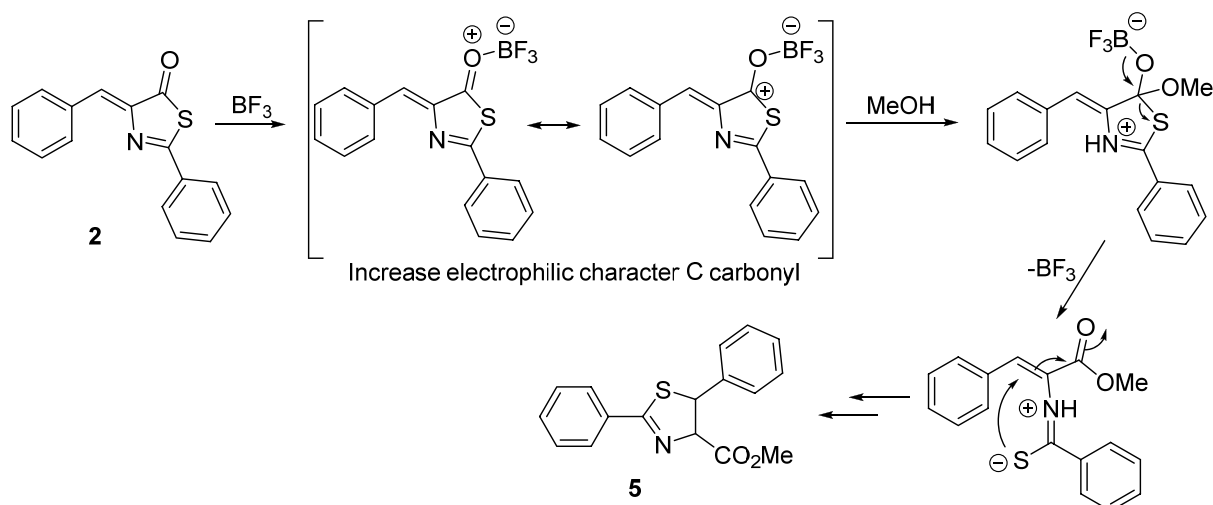
Figure 16. Mechanistic proposal for the formation of dihydrothiazoles in the presence of \text{BF}_3 .
