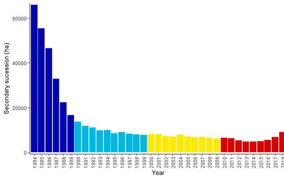
Fig. 6. Temporal evolution of SS. Colors represents the different decades.
