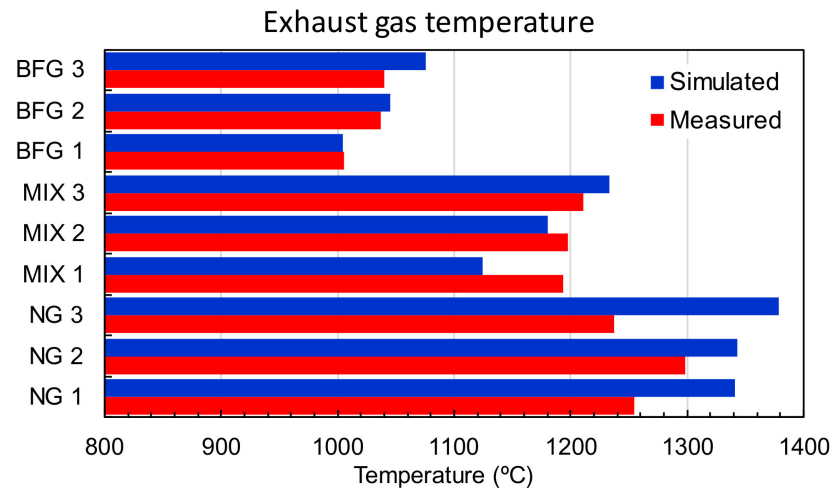
Figure 7. Comparison of exhaust temperatures measured and simulated.
