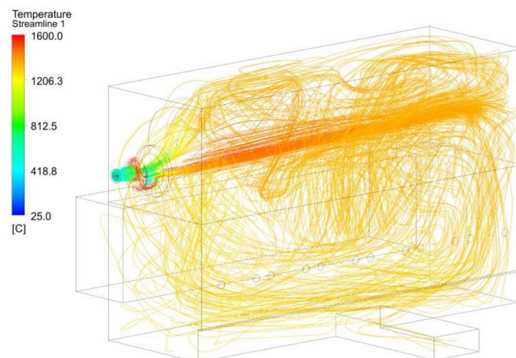
Figure 29. Temperature streamlines for the NG1 case.
