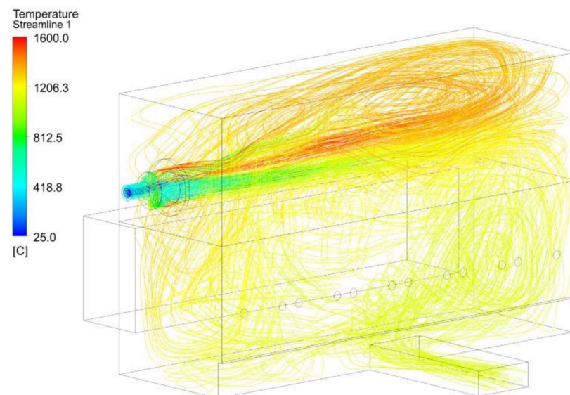
Figure 22. Temperature streamlines for the MIX 1 case.
