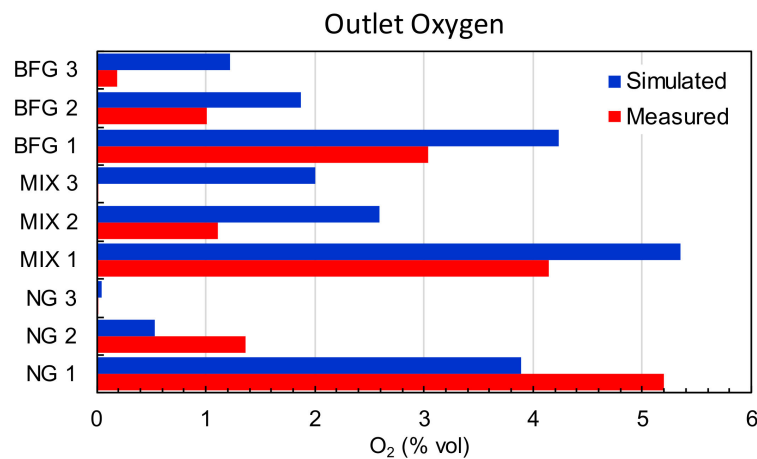
Figure 9. Comparison of oxygen concentrations measured and simulated.
