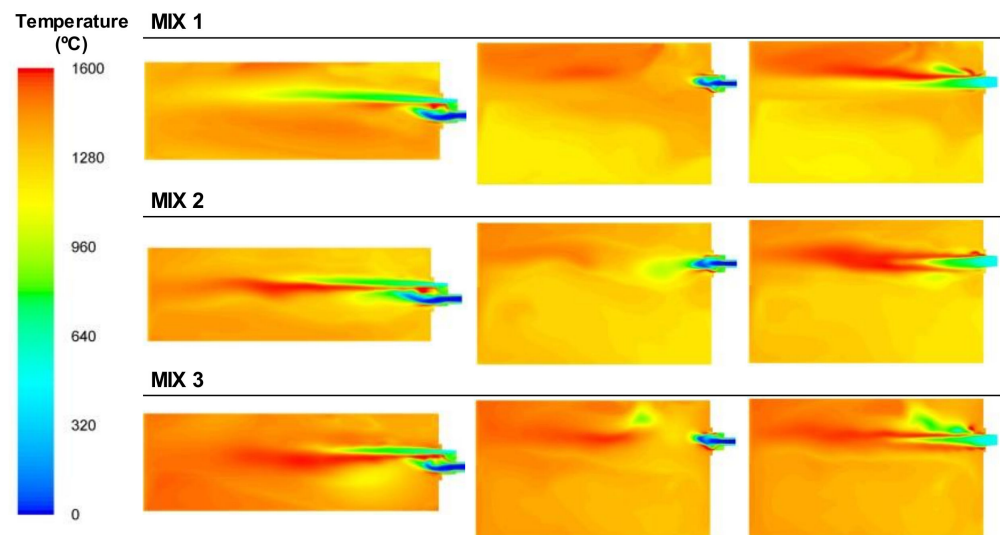
Figure 18. Contour plots of temperatures for the BFG/NG mixture cases in the XZ1, XY1, and XY2 planes.
