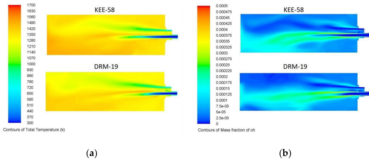
Figure 5. Comparison of the (a) temperatures and (b) OH mass fractions of the burner's central plane for the KEE-58 and DRM-19 mechanisms with BFG as fuel and an air excess of 4%.
