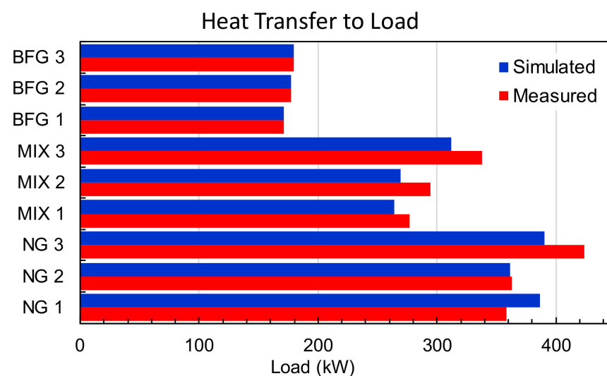
Figure 8. Comparison of transferred heat to the load measured and simulated.
