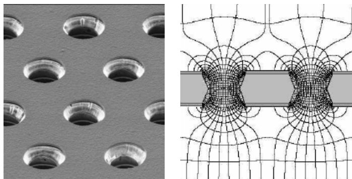
Figure 2.7: Left: microscope view of a GEM. Right: electric field configuration of a GEM.
