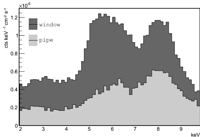
Figure 9.40: Contribution to the final spectrum through the cathode's window and the piece of pipe from detector to magnet's bore out of the shielding.
