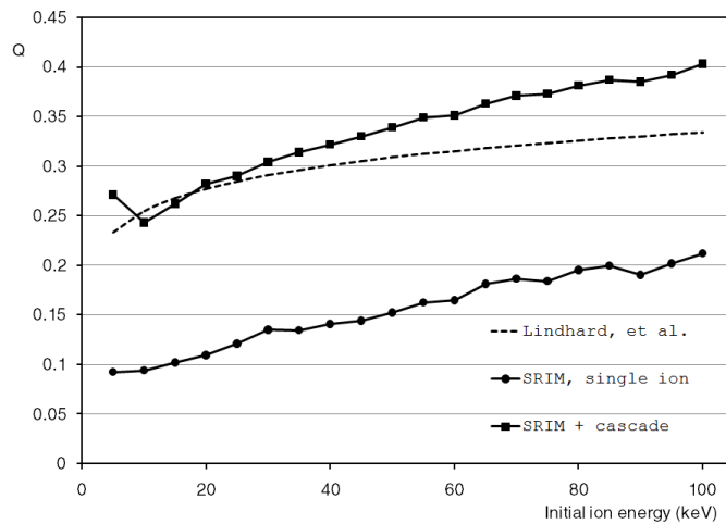
Figure 3.12: Quenching factor for Ar in Ar obtained from SRIM simulations, with and without addition of secondary recoils contribution, compared with 3.16.
