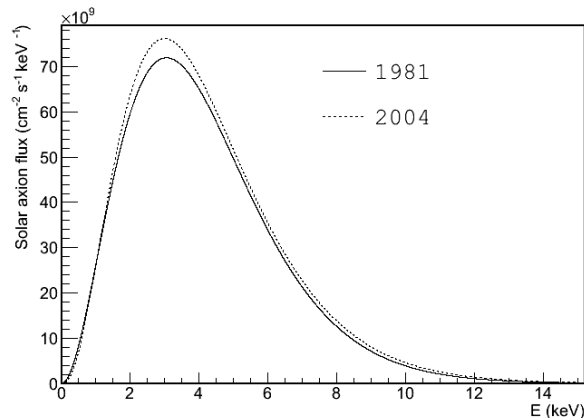
Figure 1.8: Solar axions flux spectrum. An early calculation[83] is compared with a 23 years newer one[84].
