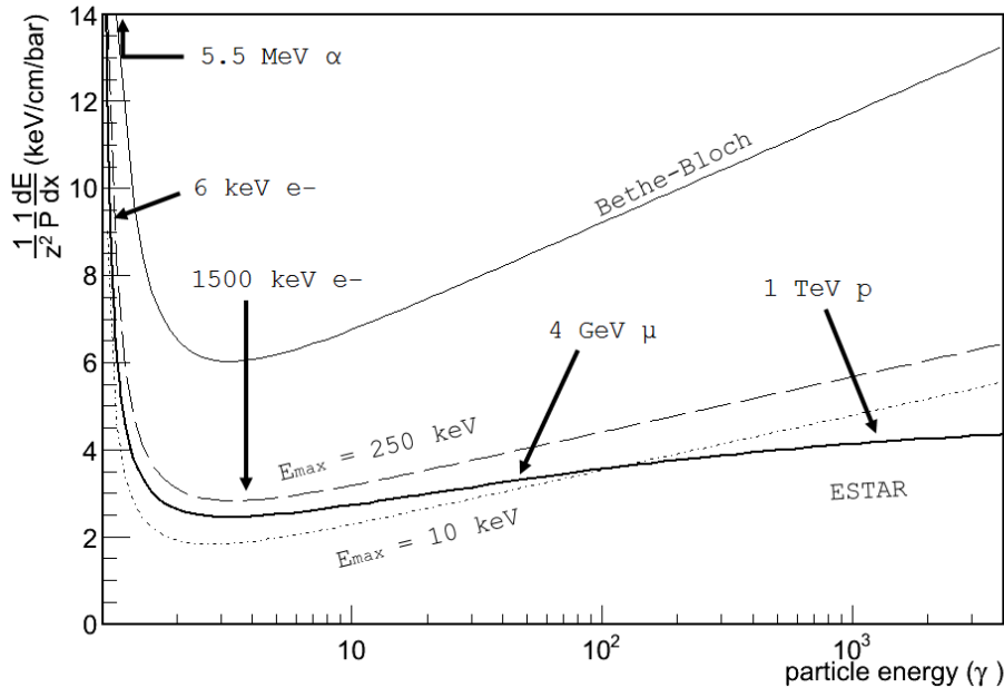
Figure 3.5: Several calculations for the stopping power in Ar. The original Bethe-Bloch formula is compared with the restricted energy loss modification for two different cuts (justified in the text) and the NIST ESTAR database. Note that ESTAR is a parametrization for electrons. Some usual incident particles are located in the plot to give a graphical idea of their Physics case: the ^{241}\text{Am} \alpha ( \beta = 0.05 ), the ^{55}\text{Fe} photoelectrons ( \beta = 0.15 ), 1500 keV electrons ( \beta = 0.97 ) as those involved in ^{136}\text{Xe} \beta\beta decay, mean energy cosmic muons ( \beta = 0.9997 ) and LHC protons ( \beta = 0.9999996 ).
