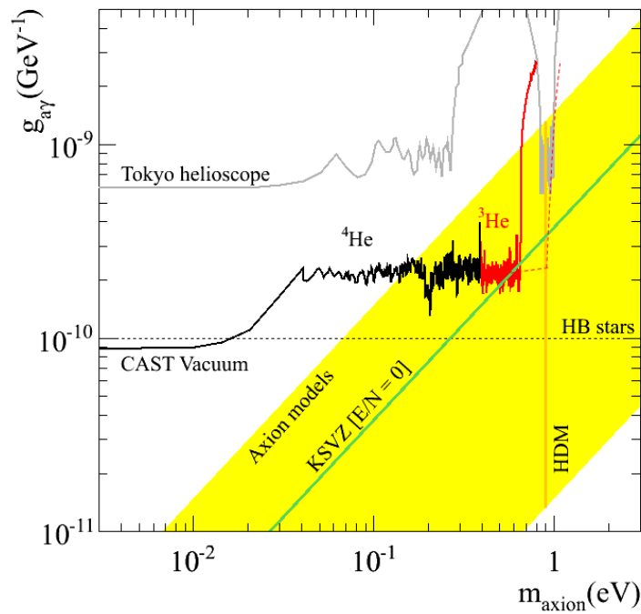
Figure 8.2: CAST exclusion plot for axions. The Vacuum phase or Phase I (2003–2004), yields a more restrictive limit for the coupling constant at lower axion masses). The 4 He Phase II (2005–2006), also in black, presents some spikes due to the discrete changes of cold-bore pressure. A partial result of the 3 He Phase II (2007–2011) obtained mainly from the 2008 data is plotted too. The red dashed line represents final 3 He results expectation; the measurements were finished in 2011 reaching a pressure which made CAST sensitive to 1.18 eV axions (still pending on final analysis).
