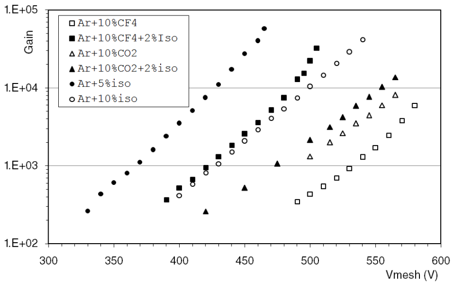
Figure 4.25: Gain curves for bulk micromegas using different gas mixtures. The last (highest) point of each series corresponds to the maximum stable gain.
