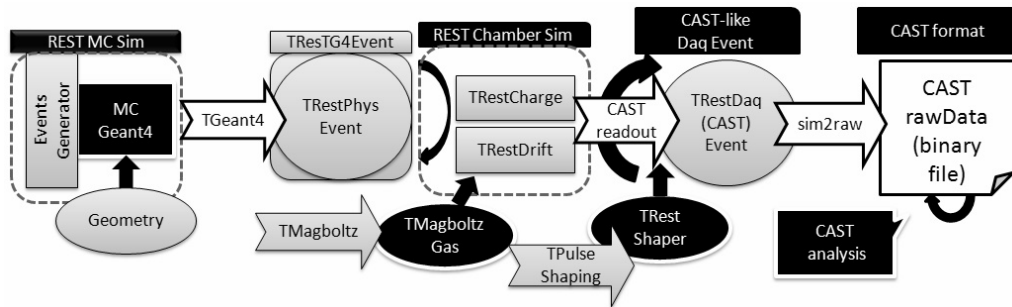
Figure 9.1: General sketch of the complete simulation chain. With a specific description of the sunrise set-up geometry, the usual simulation chain described in chapter 9 is used to produce TRestPhysEvents which have drifted to the micromegas. Then a new event holder class, TRestDaqCASTevent has been implemented to produce and hold the DAQ-like data. The sim2raw program yields the data in the proper format. The three levels of data processing are accessible at every moment: TRestG4Events with the information rescued from the GEANT4 simulation (see section 6.7), TRestDaqCASTEvents (see section 9.1.2) with raw-data as it was generated (not subjected to analysis interpretation) and, finally, analysed events (see section 8.3.1), that the discrimination routines will consider.
