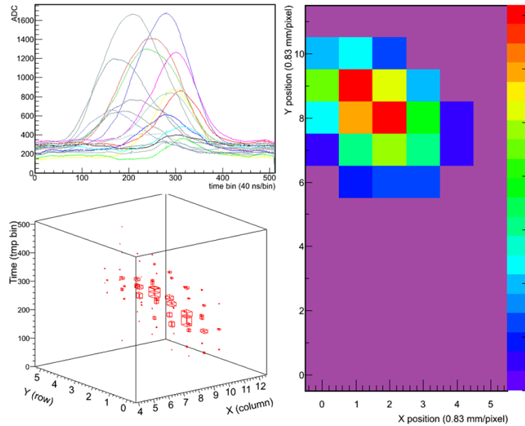
Figure 5.13: ^{241}\text{Am} 5.5 MeV \alpha event in pure Ar at 1.23 bar and E_{drift} = 20 V/cm. The mean length of \alpha tracks is 4.3 cm and longitudinal \sigma for 6 cm drift is 8.6 mm. T2K electronics configuration: 25 MHz sampling rate and 1 \mu\text{s} shaping time.
