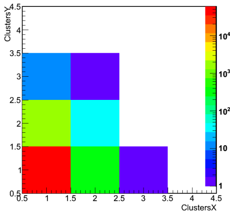
Figure 8.16: Identified clusters per event in X and Y axis in a ^{55}\text{Fe} calibration. The fact that events with two clusters only in one axis is much higher than events with two clusters found in both axis points to statistical fluctuation to have produced the secondary clusters, in that case they could be ignored. That can have an important effect in software efficiency for lower energy events.
