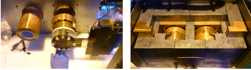
Figure 8.8: Left: early step during sunset 2012 installation. The auto-shielded copper pipe with an inner Teflon coating is visible in the left (Jura) bore; in the right bore (Airport) the detector installation using Teflon and Delrin screws, nuts and gaskets, the new copper gas connections and top piece of the new inner copper shielding which fits the pipe. Right: later step during shielding mounting process showing the careful design to adjust copper shielding to detectors (closing as much as possible every outlet), Faraday cage and lead layer. Note that not only detectors but also the pipe are shielded, thus the detectors' cavity can only be accessed through a long, strongly shielded and radiopure pipe.
