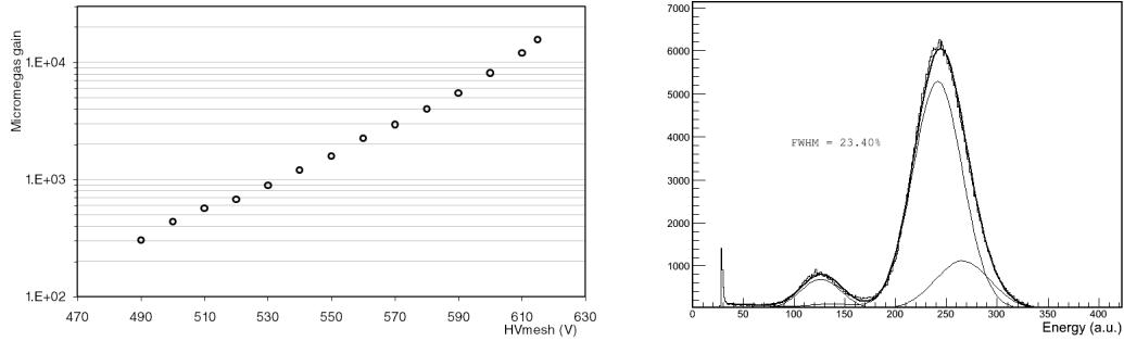
Figure 7.14: Performance of Ar/ \text{CF}_4/i\text{C}_4\text{H}_{10} 73/25/2 in a bulk micromegas. Left: gain curve, with E_{\text{drift}} = 800 V/cm. The highest voltage point corresponds to the highest achievable stable gain. Right: resolution at optimum operational point: E_{\text{drift}} = 600 V/cm and \text{HV}_{\text{mesh}} = 580 V (Amplification gap is 128 \mu\text{m} ).
