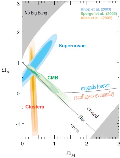
Figure 1.4: Three independent sets of observations: high-redshift supernovae, galaxy cluster inventories, and the CMB, converge nicely. The dark grey corner (down right) corresponds to a too recent Big Bang. Figure extracted from [24].
