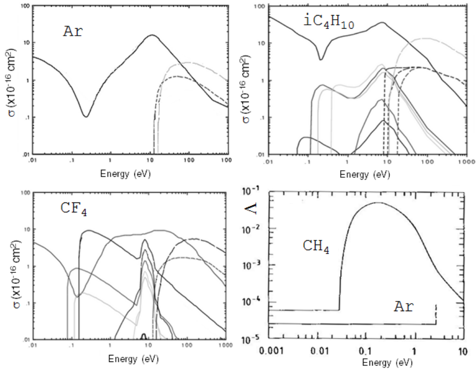
Figure 4.3: Cross sections for effective momentum transfer of electron with Ar, isobutane and CF 4 , extracted from [150]. The solid line, which is continuous along the energy range and shows the Ramsauer dip around 0.1 eV, corresponds to the elastic cross section. The rest of solid lines are vibrational modes. The short dashed lines curves, which raise about 10 eV, are excitation cross sections. The long dashed ones, which are activated only with slightly higher energies, corresponds to the ionization cross sections. The last plot, taken from [116] shows a comparison of the inelasticity of the collisions of Ar and methane.
