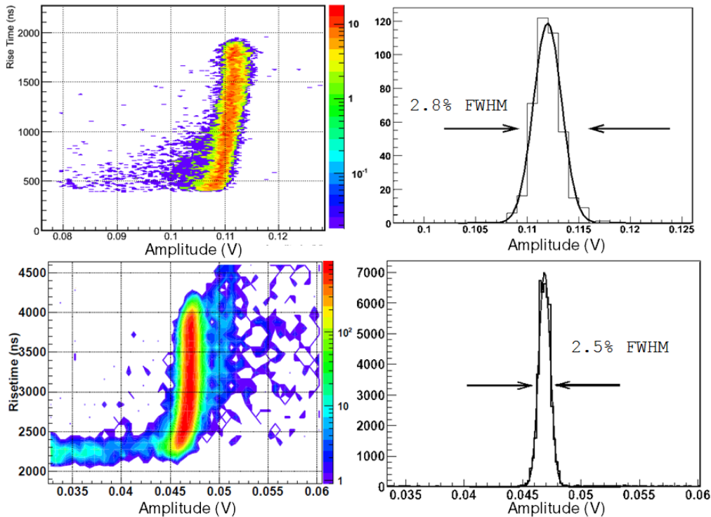
Figure 5.5: Risetime vs amplitude plots and energy spectra of ^{241}\text{Am} \alpha for pure xenon in up : Saclay's set-up at 2 bar with E_{drift} = 480\ \text{V/cm} [161] and down : Zaragoza's set-up at 4 bar with E_{drift} = 300\ \text{V/cm} [155]. Note the drift field is lower in the second case (specially the reduced field E/P ) while the maximum drift distance has been doubled from 3 to 6 cm. However, the upper spectrum has been obtained applying the constraint 1800 < \text{risetime} < 2000\ \text{ns} and in the downer the whole pulses distribution is fitted.
