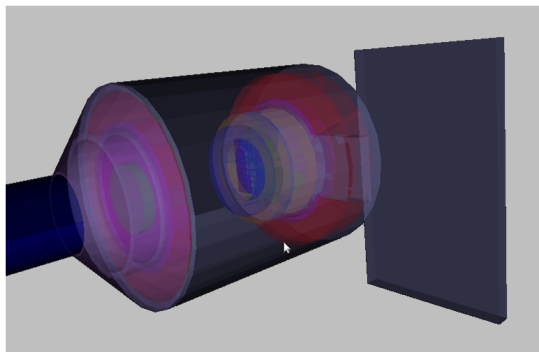
Figure 9.3: Left: GEANT4 SRMM geometry, detail of the shielding and pipe connection, to be compared with figure 8.7 left. Right: sketch of the shielding's layers.
