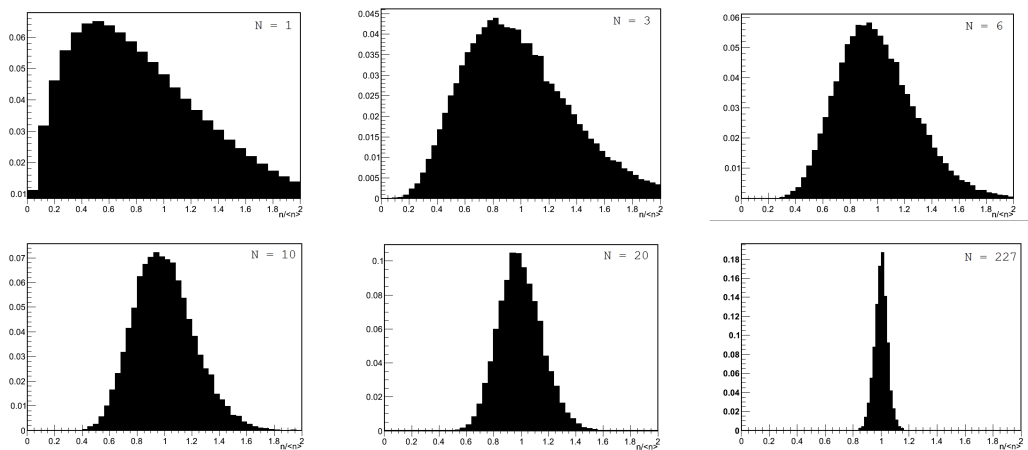
Figure 6.14: Distributions of the sum of N avalanches yield with single avalanche simulated with a Polya( m = 2, \bar{N} = 100 ).
