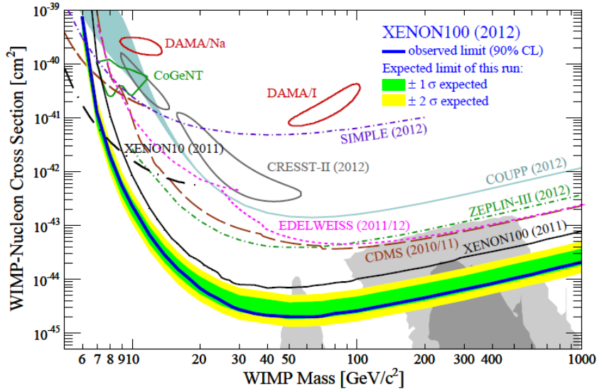
Figure 1.6: WIMPs current exclusion plot summary for spin-independent WIMP-nucleon scattering and standard DM galactic halo[45] as published by XENON100[44], currently the most sensitive DM experiment. The remarked regions correspond to DAMA and other WIMP claims (by CoGeNT and CRESST), in principle excluded by XENON100. The XENON100 immediate prospects are exploring the SUSY favoured region (grey 1\sigma/2\sigma contours). The plot shows the amazing improvement in experiments sensitivity about 4 orders of magnitude during the last decade, since in the early 2000's the DAMA region was not covered.
