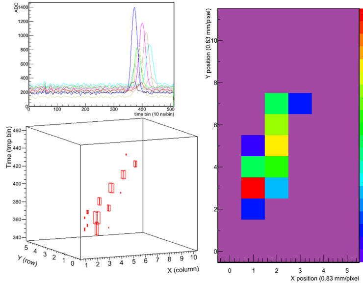
Figure 5.12: ^{241}\text{Am} 5.5 MeV \alpha event in Ar with 2% i\text{C}_4\text{H}_{10} at 1 bar and E_{drift} = 30 V/cm. The mean length of the \alpha tracks is 5.3 cm. T2K electronics working at fastest mode: 100 MHz sampling rate and 100 ns shaping time. Right: individual pixels maximum amplitude. Top left: recorded pulses. Bottom left: event reconstruction.
