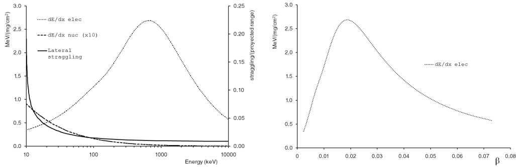
Figure 3.7: Left: Stopping power for He ions in He gas from SRIM tables. The nuclear stopping power has been amplified ten times. The lateral straggling is also represented for ions with this initial energy. Right: electronic stopping power as function of velocity for the same energy range. Note the linear regime around 0.01 \lesssim \beta predicted by LSS-theories.
