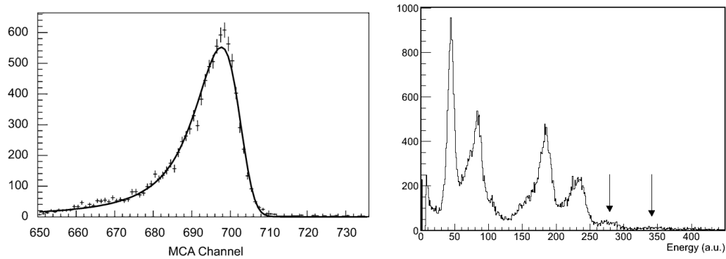
Figure 5.2: ^{241}\text{Am} spectra [161] in \text{Ar}/i\text{C}_4\text{H}_{10} 98/2. Left: 5.5 MeV ^{241}\text{Am} \alpha at 4 bar, a simple fit yields 1.8% FWHM and 0.7% FWHM is the deconvoluted value (see the text). Right: low energy 26.4 keV \gamma and 13.9, 17.7 and 21.0 keV X-rays; in addition 3.0 and 6.1 keV fluorescences from the chamber, taken at 2 bar.
