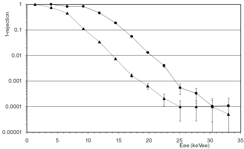
Figure 7.9: \gamma /electron events rejection via size cut with the chambers explained in the text: circles for a 3 cm height chamber filled with Ar/ i\text{C}_4\text{H}_{10} / \text{CF}_4 90/5/5% and triangles for another with 10 cm and an ideal \sigma = 100\ \mu\text{m cm}^{1/2} . 10^{-4} is the statistics limit for each group of electron events simulated.
