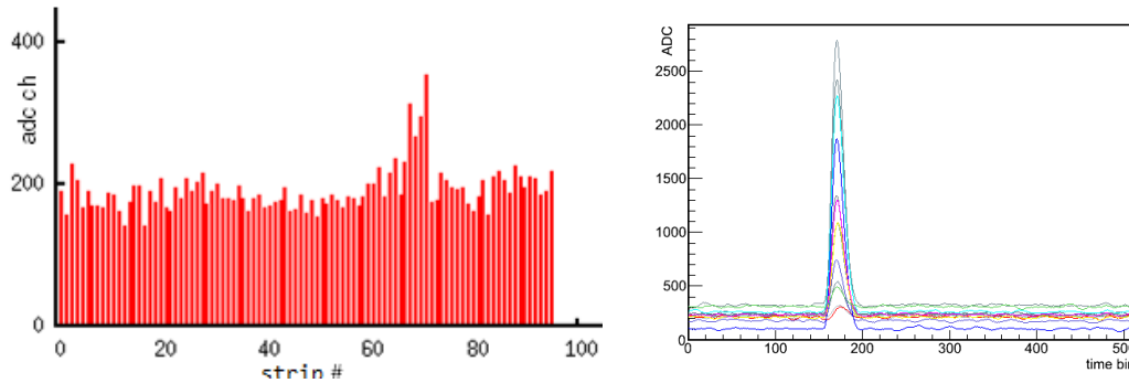
Figure 11.5: Strips signals upgrade. ^{55}\text{Fe} 6 keV X-ray signals in a CAST micromegas as seen by the classic Gassiplex card (left) and the T2K electronics (right).
