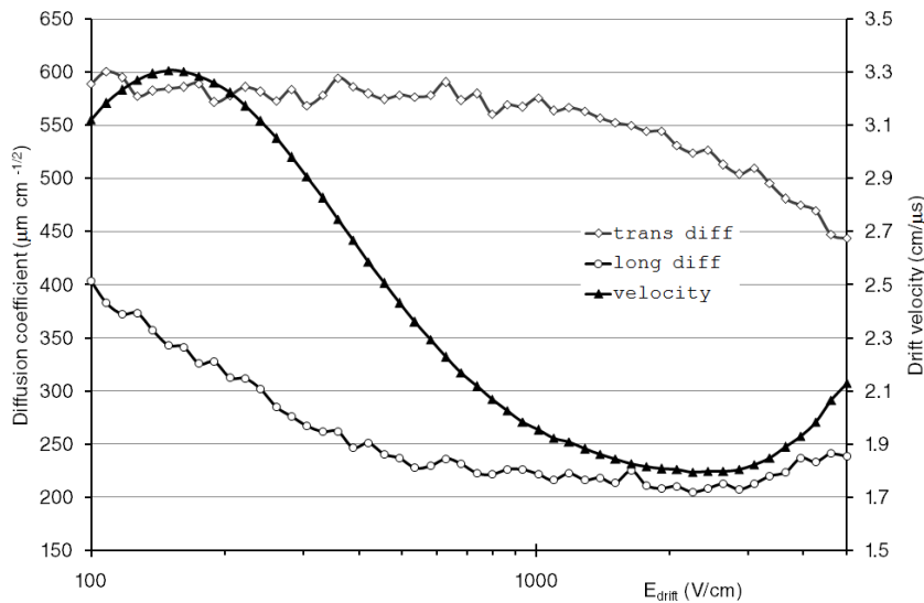
Figure 9.5: Gas properties as stored in the TMagboltzGas object used in the simulations. The CAST operation point is in the lowest drift field.
