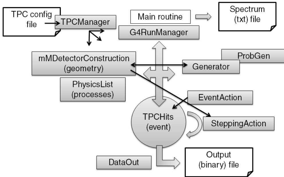
Figure 6.6: Elemental sketch of the RESTSoft GEANT4 application. G4RunManager is the GEANT4 class that coordinates the rest of them. The configuration options loaded by the TPCManager are available at any point of the program. Together with TPCManager , ProbGen , TPCHits and DataOut are the only classes that do not inherit from a GEANT4 prototype.
