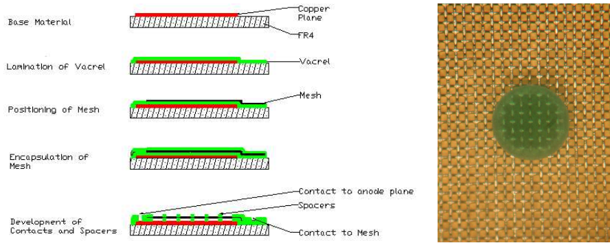
Figure 2.4: Left: sketch of the bulk manufacturing process[101]. Right: detail of the iron woven mesh showing one of the vacrel pillars.
