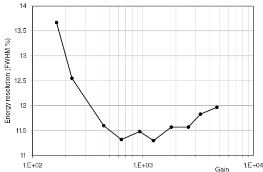
Figure 4.27: Resolution vs gain, taken with a CM microbulk in Zaragoza. No very high gains were tried during that test, so as not to risk the microbulk. Equivalent curves showing further resolution degradation at high gain can be found, for instance, in [100].
