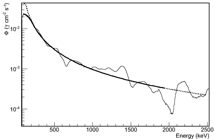
Figure 9.36: Extracted \gamma continuum flux after process and fit. The dashed line is an interpolation of the potential fit 9.8 beyond its range.
