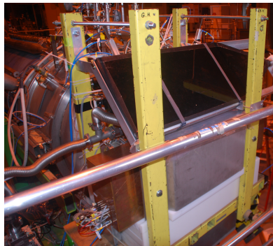
Figure 8.9: 2012 sunset final installation (see the Faraday cages backs with the electronic connections) showing the cosmic muon veto (plastic scintillator) over the shielding. The veto is mounted in 50^\circ because of space availability with present vacuum system.
