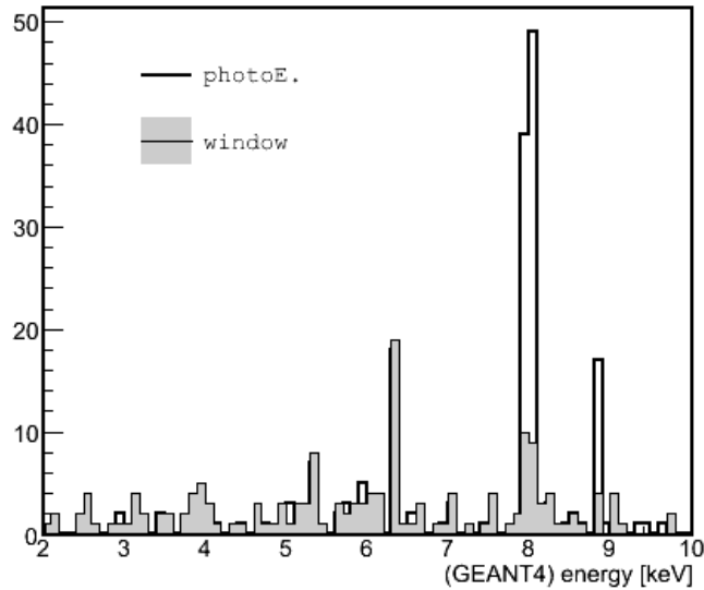
Figure 9.27: Partial final spectra for the E_\gamma = 2614 keV run selecting photoelectric (42.8% [2-10 keV]) and window (40.1% [2-10 keV]) events. Note the 6 keV peak matches, while the copper ones have other important contributions.
