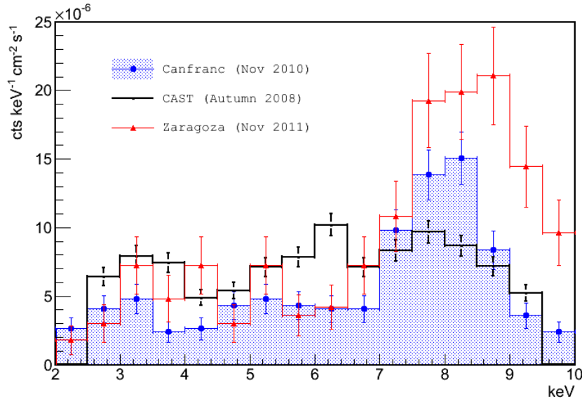
Figure 10.17: Three background spectra registered by the M10 microbulk detector: in CAST sunrise (R11) side and, with tests CAST-like set-up, underground (R2) and at surface (R12).
