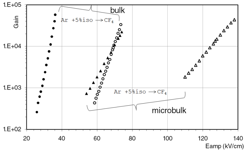
Figure 4.24: Comparison of gain curves for bulk (circles) and microbulk (triangles) micromegas in Ar/ i\text{C}_4\text{H}_{10} 95/5 (filled markers) and \text{CF}_4 (empty markers). The maximum gain cannot be directly compared because different prototypes were used.
