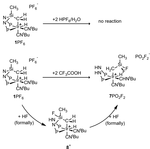
Scheme 6. Reaction of [\text{IrH}\{\kappa^3\text{C},\text{P},\text{P}'\text{-SiNP-H}\})(\text{CN}^t\text{Bu})_2][\text{PF}_6] with \text{HPF}_6 or \text{CF}_3\text{COOH} .
