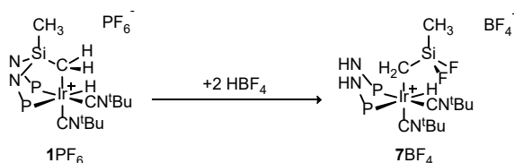
Scheme 5. Reaction of [\text{IrH}\{\kappa^3\text{C},\text{P},\text{P}'\text{-(SiNP-H)}\}(\text{CN}^t\text{Bu})_2][\text{PF}_6] with HBF 4 .
