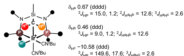
Figure 4. Selected 1 H and 31 P NMR data for the IrHCH 2 moiety of 1 + .
