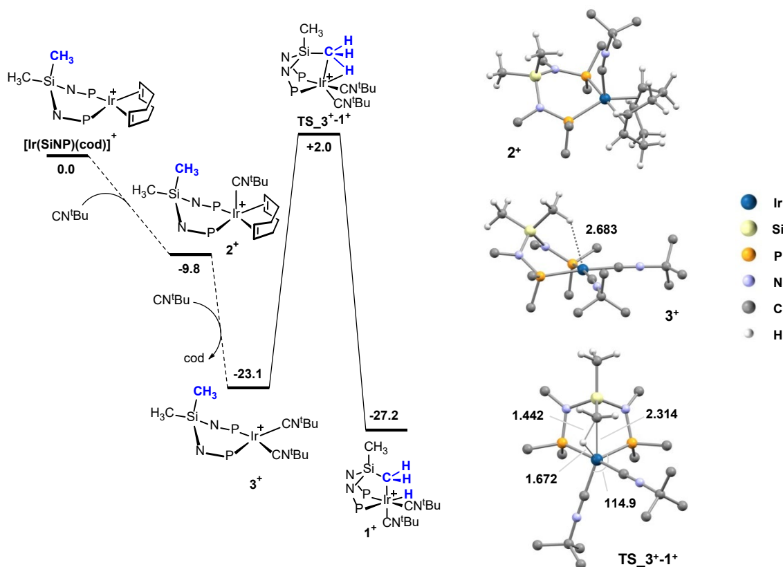
Figure 5. (left) Relative Gibbs free energy profile ( \text{kcal}\cdot\text{mol}^{-1} ) of the reaction \text{Ir}(\text{SiNP})(\text{cod}) + 2 \text{CN}^t\text{Bu} \rightarrow 1^+ + \text{cod} (M06/def2tzvp//B3PW91-GD3BJ/def2svp, 298 K, 1 atm); (right) view of the calculated structures of 2^+ , 3^+ and \text{TS}_{3^+-1^+} with selected interatomic distances ( \text{\AA} ) and angles ( ^\circ ) (for clarity, most hydrogen atoms are omitted and only the ipso carbon atoms of the phenyl and tolyl moieties are shown).
