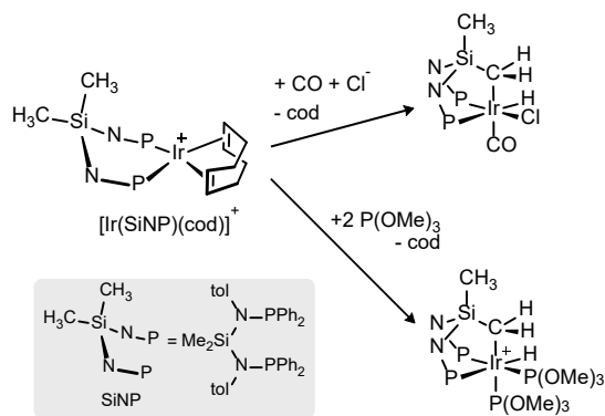
Scheme 1. Reactivity of [\text{Ir}(\text{SiNP})(\text{cod})]^+ towards CO or \text{P}(\text{OMe})_3 .
