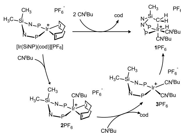
Scheme 2. Reaction of [\text{Ir}(\text{SiNP})(\text{cod})]^+ with \text{CN}^t\text{Bu} showing the observed intermediates.
