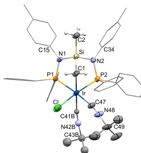
Figure 6. ORTEP plot of [\text{IrCl}\{\kappa^3\text{C},\text{P},\text{P}'-(\text{SiNP}-\text{H})\}(\text{CN}^t\text{Bu})_2]^+ ( 4 + ). For clarity, most hydrogen are omitted and the tolyl and phenyl rings are represented in a wireframe style. Selected bond lengths ( \text{\AA} ) and angles ( ^\circ ) are given in ESI.
