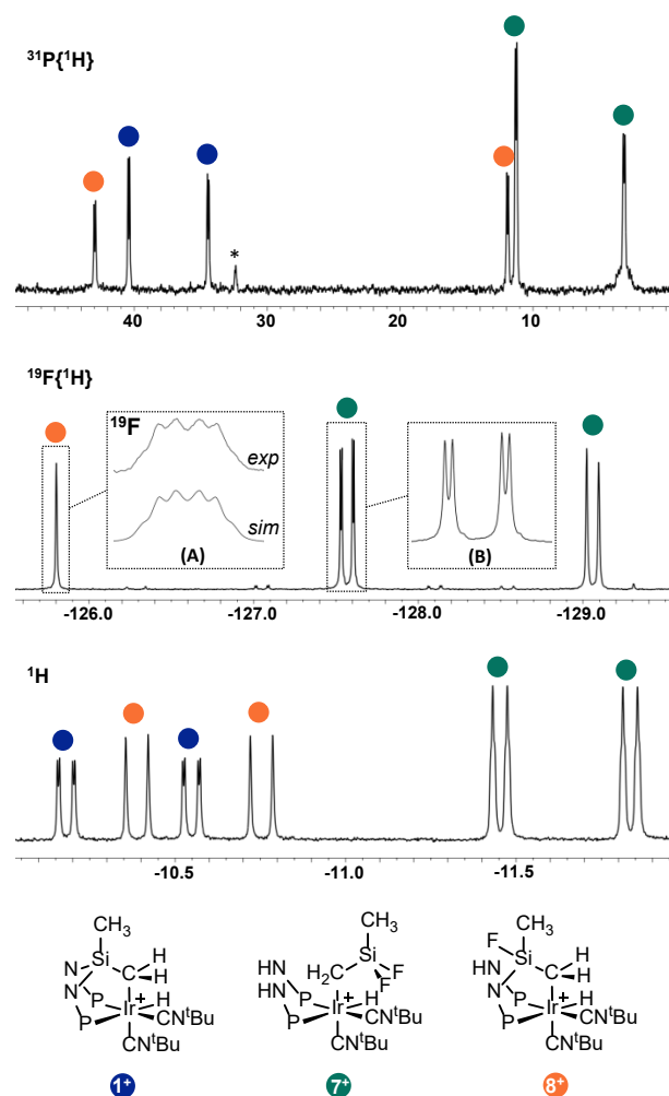
Figure 8. Selected areas of the ^1\text{H} , ^{19}\text{F} , ^{19}\text{F}\{^1\text{H}\} and ^{31}\text{P}\{^1\text{H}\} NMR spectra of the mixture resulting from the reaction of 1PF 6 with \text{CF}_3\text{COOH} in \text{CD}_2\text{Cl}_2 after 24 h with the proposed assignment. Inset A shows the experimental and simulated ^{19}\text{F} signal at -125.8 ppm of 8 + . Inset B shows the expanded view of the ^{19}\text{F}\{^1\text{H}\} signal at -127.5 ppm of 7 + . * unassigned.
