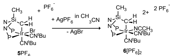
Scheme 4. Bromide abstraction from [\text{IrBr}\{\kappa^3\text{C},\text{P},\text{P}'\text{-(SiNP-H)}\}(\text{CN}^t\text{Bu})_2]^+ ( 5^+ ).
