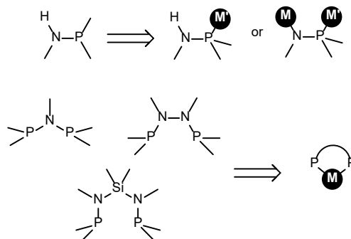
Figure 1. Selected amino-phosphane scaffolds and related metal-ligand structures.
