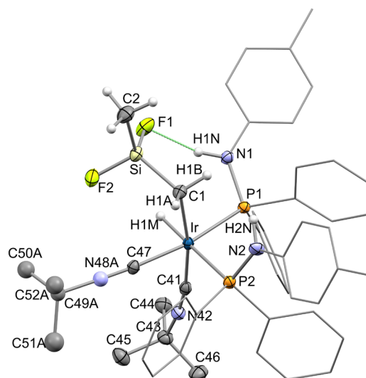
Figure 7. ORTEP plot of [\text{IrH}(\text{CH}_2\text{SiF}_2\text{Me})(\text{HNP})_2(\text{CN}^t\text{Bu})_2]^+ ( 7^+ ). For clarity, most hydrogen are omitted and the tolyl and phenyl rings are represented in a wireframe style. Selected bond lengths (Å) and angles (°) are given in ESI.
