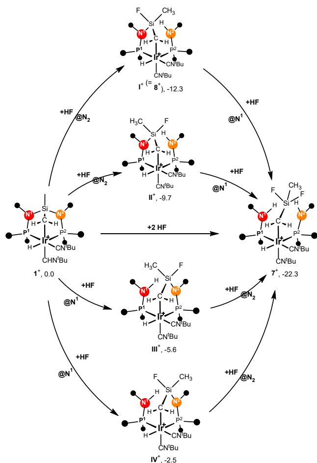
Figure 9. Sequential addition of HF to 1^+ showing the possible intermediates and their relative Gibbs free energies (M06/def2tzvp//B3PW91-GD3B/def2svp, 298 K, 1 atm).
