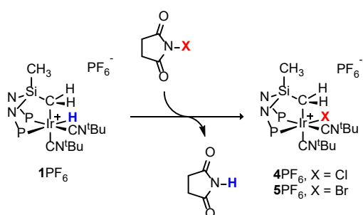
Scheme 3. Hydride-halide exchange on [\text{IrH}\{\kappa^3\text{C},\text{P},\text{P}'-(\text{SiNP}-\text{H})\}(\text{CN}^t\text{Bu})_2][\text{PF}_6] ( 1PF 6 ).
