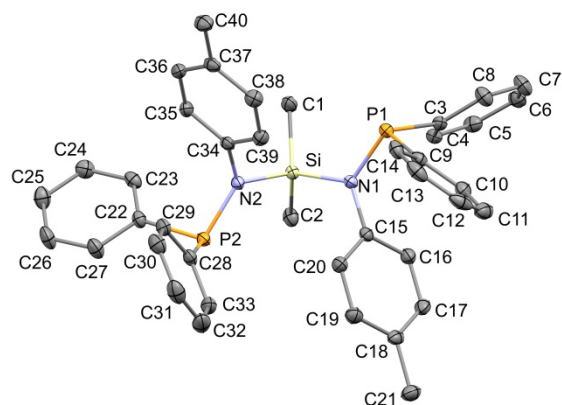
Figure 2. ORTEP plots of [\text{IrH}\{\kappa^3\text{C},\text{P},\text{P}'-(\text{SiNP}-\text{H})\}(\text{CN}^t\text{Bu})_2]^+ ( \mathbf{1}^+ ) (top) and of SiNP (bottom). For clarity, most hydrogen are omitted and the tolyl and phenyl rings are represented in a wireframe style for [\text{IrH}\{\kappa^3\text{C},\text{P},\text{P}'-(\text{SiNP}-\text{H})\}(\text{CN}^t\text{Bu})_2]^+ . Selected bond lengths (Å) and angles (°) are given in ESI.
