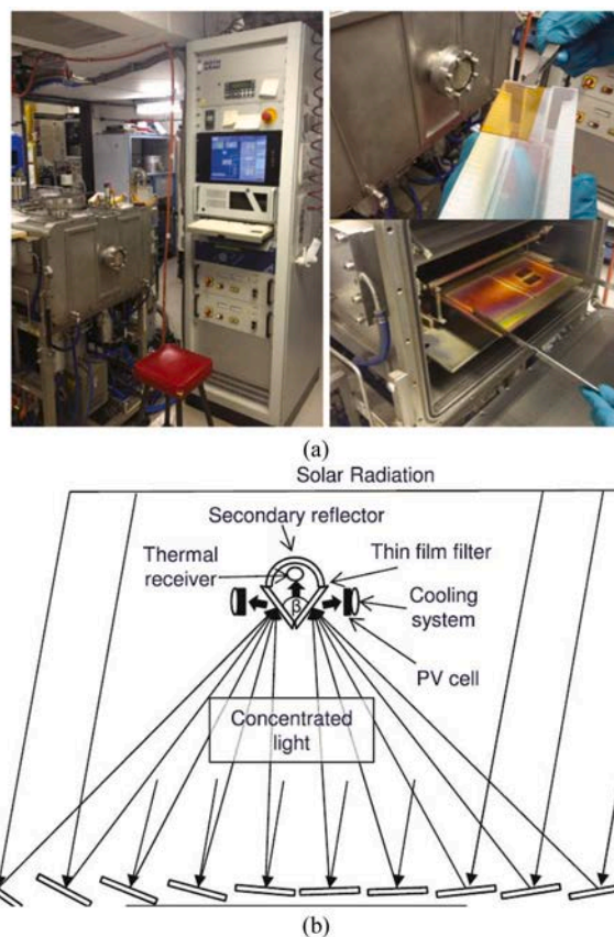
Fig. 31. Example dichroic mirror-based PV-T system: (a) plasma-enhanced chemical vapour deposition of \text{SiN}_x/\text{SiO}_2 layers on a quartz substrate (using a Roth&Rau AK400 instrument); and (b) PV-T configuration where (concentrated) short wavelengths are reflected out of the optical path towards PV cells. Images reprinted from Crisostomo et al. [419], with permission from Elsevier.
