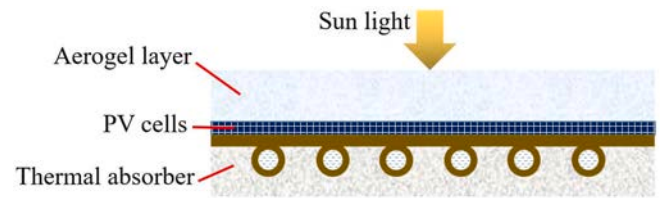
Fig. 22. Schematic of a PV-T collector covered with a highly-transparent aerogel layer [385].
