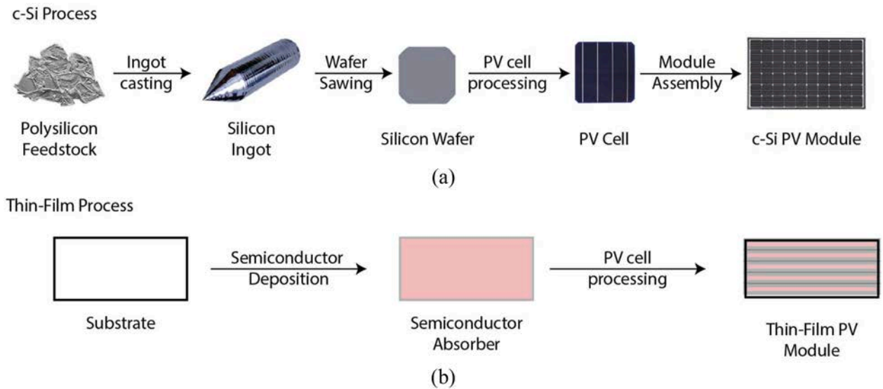
Fig. 1. Schematic diagrams showing the difference in fabrication processes for: (a) crystalline silicon solar cell; and (b) thin-film solar cell.
