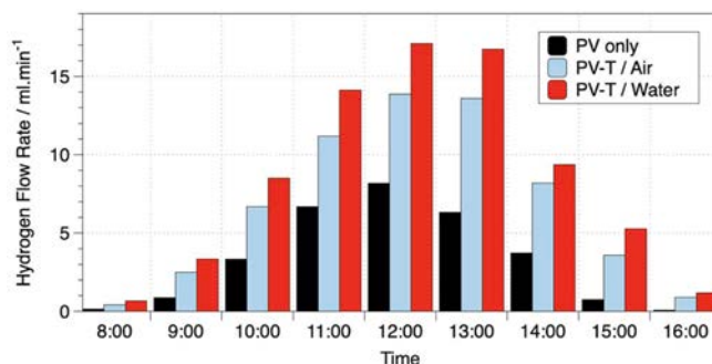
Fig. 58. Hydrogen flow rate from three combinations of PV panel and electrolyser: conventional PV panel, air-based PV-T collector and water-based PV-T collector at a mass flow rate of 0.011 kg/s. Data derived from Ref. [85].
