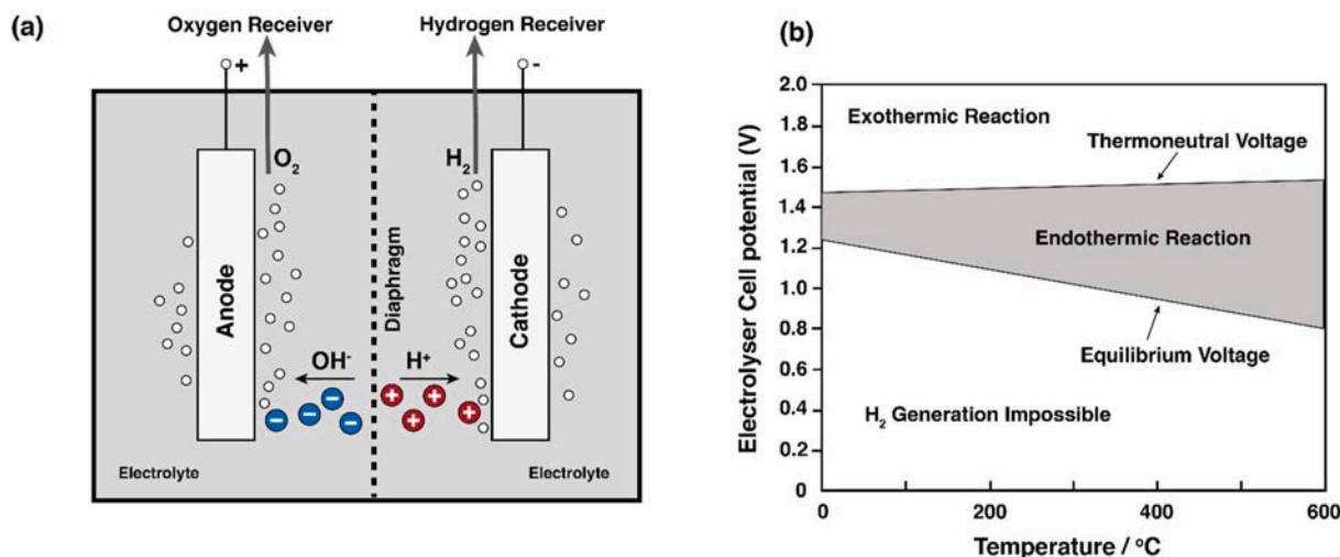
Fig. 57. (a) Schematic diagram of electrolyser; and (b) electrolyser reaction regimes plotted as a function of cell potential and temperature. Figure reproduced from Zeng and Zhang [617].
