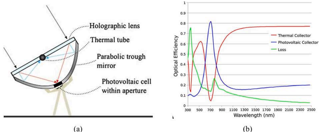
Fig. 32. (a) CPV-T collector design; and (b) calculated optical efficiency curves. Reused from Vorndran et al. [438], with permission from Wiley and Sons.
