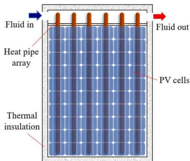
Fig. 11. Structure of flat plate heat-pipe PV-T collector. Figure reproduced from Pei et al. [173] with permission from Elsevier (Copyright 2011 Elsevier).
