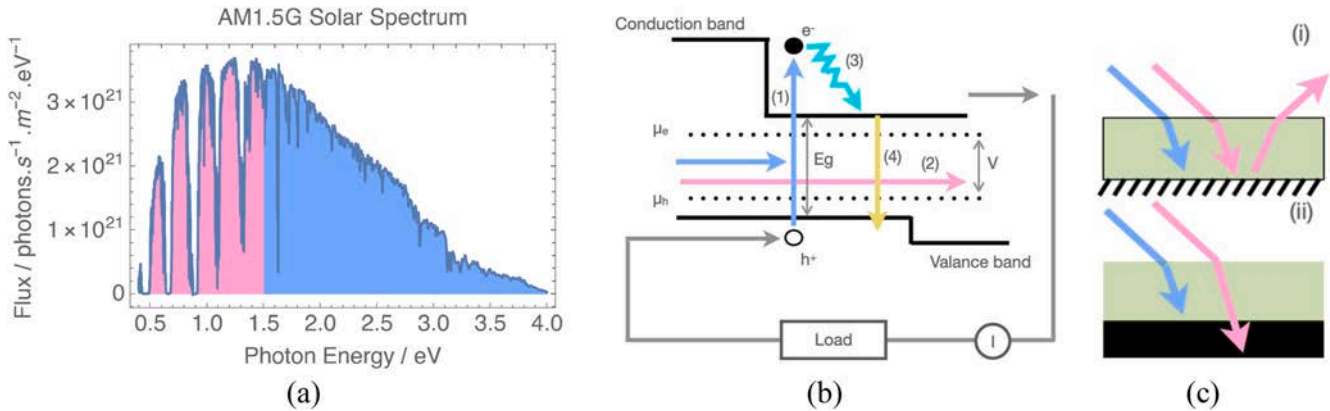
Fig. 2. (a) AM1.5G solar spectral flux b(E) plotted as a function of photon energy with an illustrative band-gap energy of 1.5 eV. (b) Schematic of a single junction solar cell of band-gap E_g showing four fundamental processes: (1) absorption of light above the band-gap energy ( E_g ); (2) transmission of light below the band-gap energy; (3) thermalization of excess energy; and (4) radiative recombination. (c) Two configurations for a PV device: (i) semiconductor absorber with rear mirror; and (ii) semiconductor absorber with the rear absorber.
