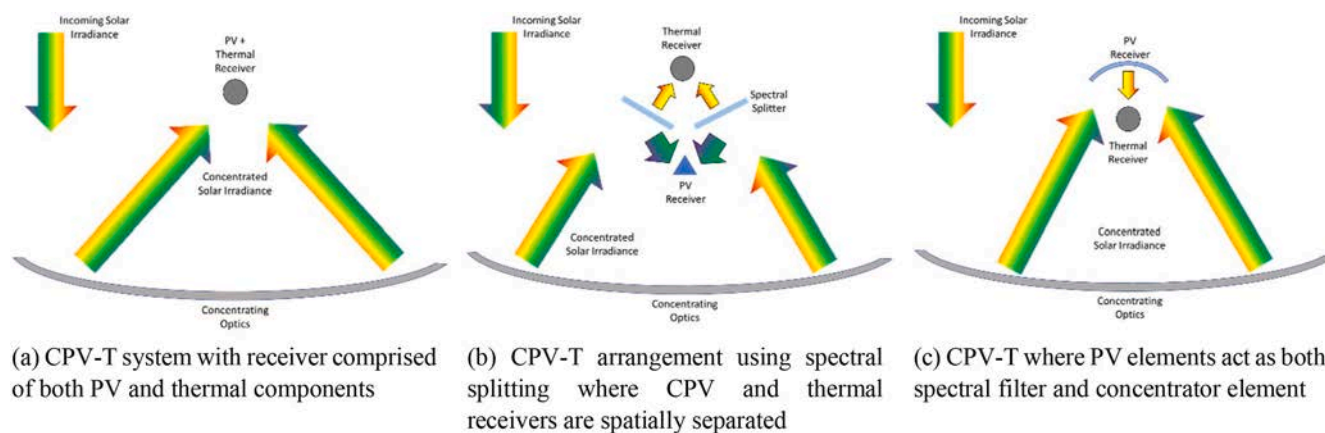
Fig. 16. Schematics of the most common types of CPV-T collectors.
