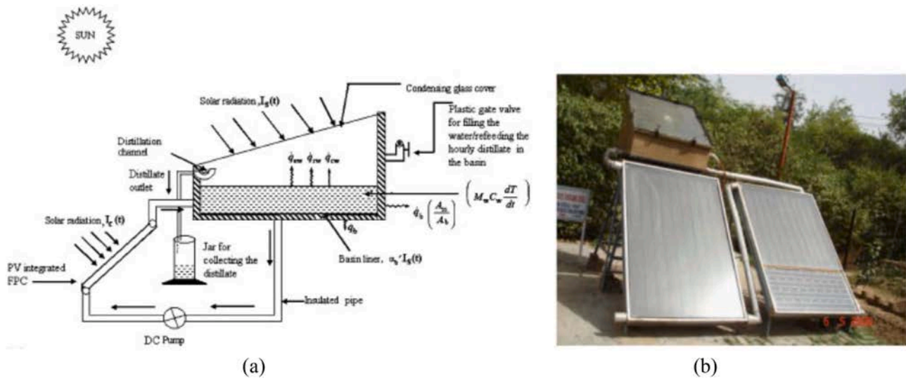
Fig. 54. (a) Schematic; and (b) photograph of an active solar still coupled to a hybrid PV-T collector. Images reprinted from Kumar and Tiwari [586], with permission from Wiley.
