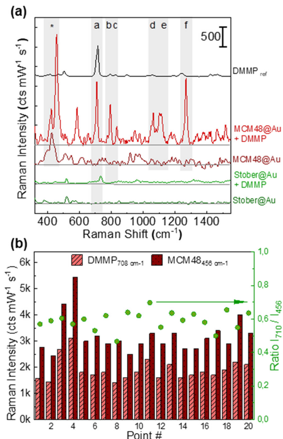
Fig. 4 (a) Average SERS spectra of DMMP (2.5 ppmV) recorded on the MCM48@Au and Stober@Au supported films compared to the Raman fingerprint of pure DMMP in the liquid phase and blank MCM48@Au and Stober@Au samples, respectively. The characteristic Raman band of MCM48-NH 2 used as a Raman internal standard is labelled with *. (b) Spatial distribution of the DMMP peak (at 710 cm -1 ) and MCM48 (at 456 cm -1 ) over 20 different points of the surface of the MCM48@Au substrate. Right axis (green dots): SERS intensity ratio between peak 710 cm -1 of DMMP and 456 cm -1 of MCM48.
