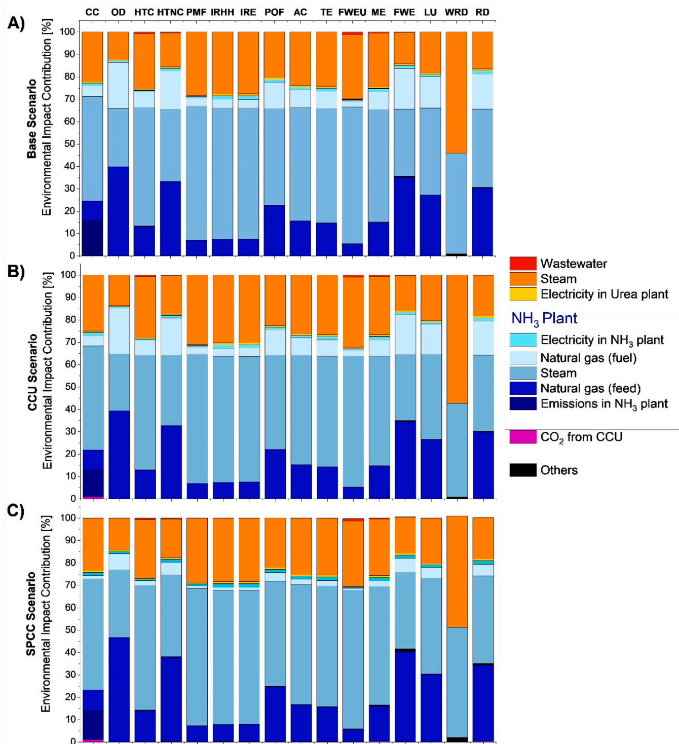
Fig. 6. EI contribution [%] of the selected input/outputs in each case study of urea production. A) Base scenario. B) Scenario with CCU and C) Scenario SPCC.
