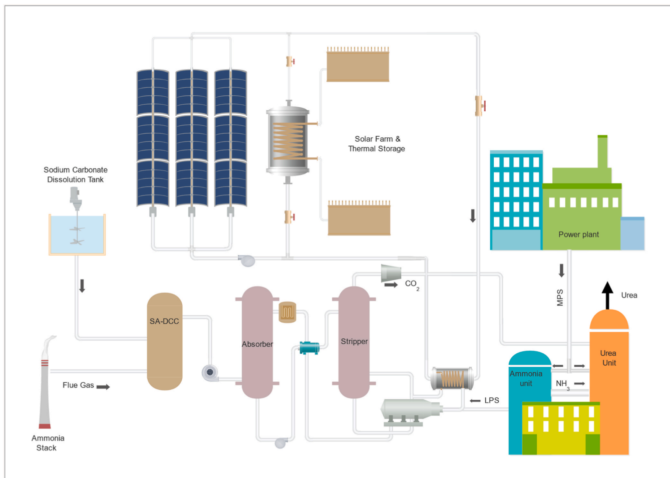
Fig. 2. Schematic of the SPCC system.
