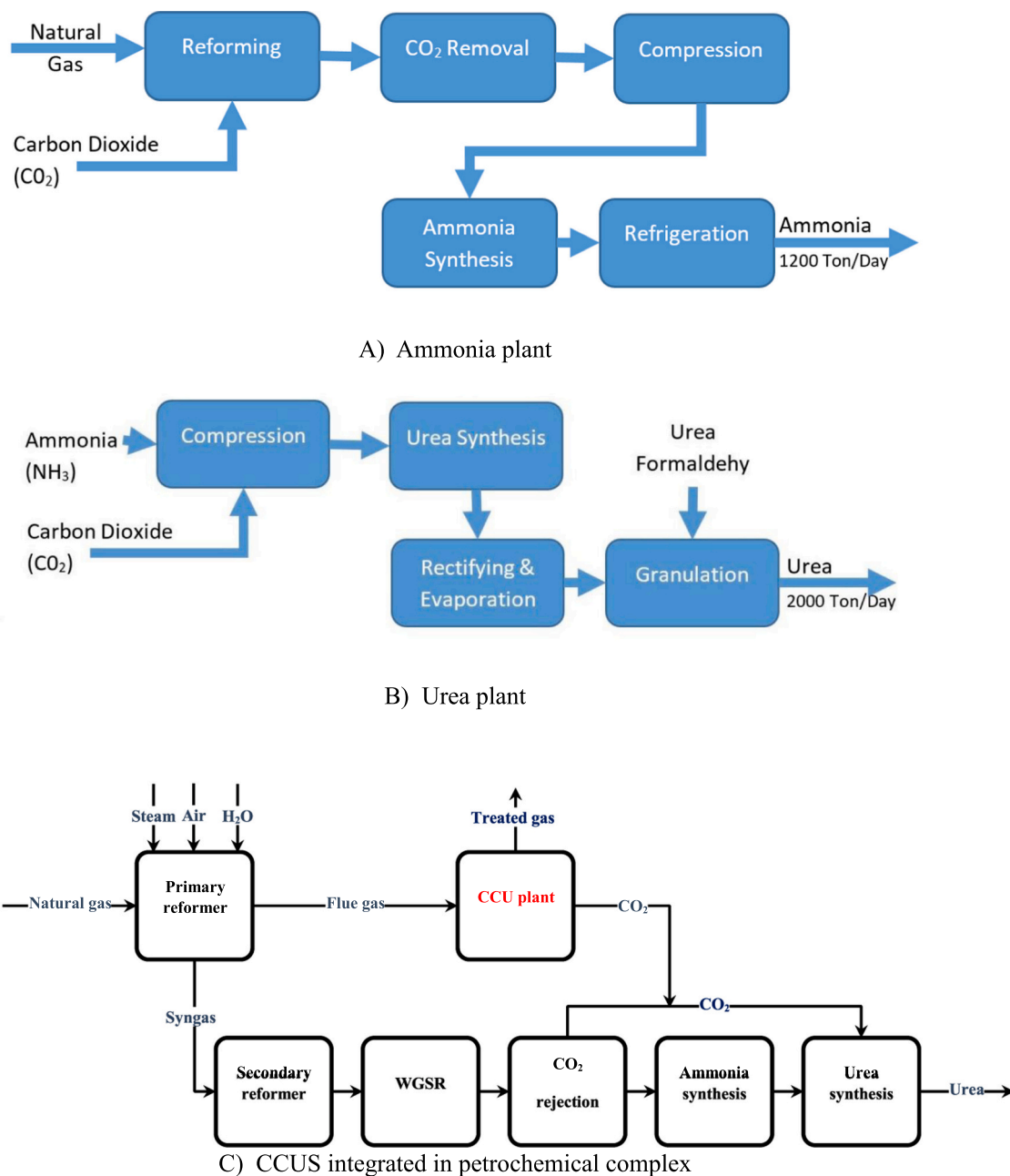
Fig. 1. Block flow diagram of the case study. A) Ammonia plant B) Urea plant C) CCUS integrated in petrochemical complex.
