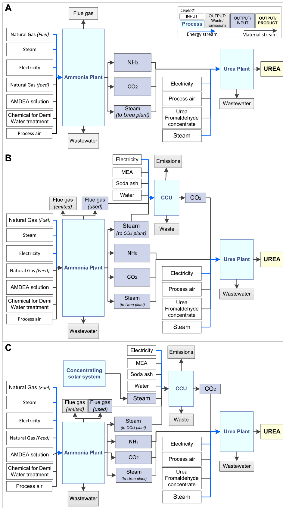
Fig. 3. Flowchart of the LCA boundaries for the three studied scenarios. A) Base scenario. B) CCU scenario. C) SPCC scenario.
