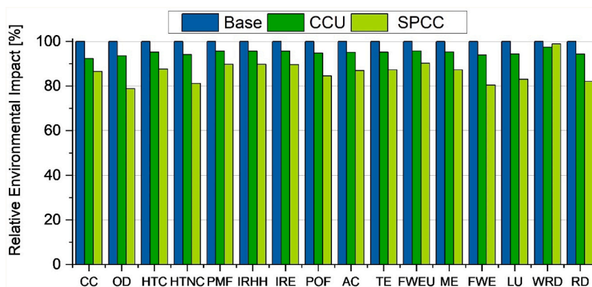
Fig. 4. LCA characterization results. Relative EIs of the three scenarios per 1 kg of urea production.
