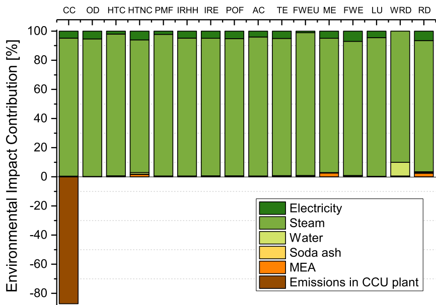
Fig. 5. CCU unit stand-alone LCA analysis. Relative contributions to CO 2 production in the CCU unit.
