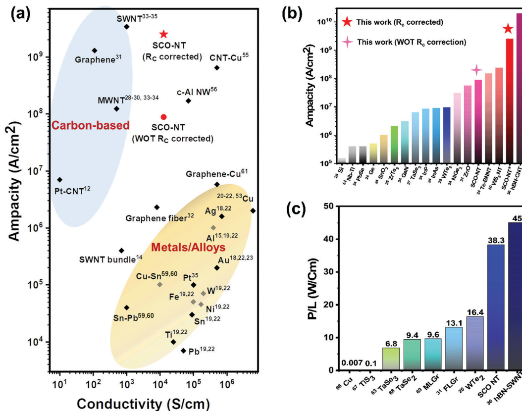
Fig. 6 (a) Ashby plot of ampacity vs conductivity for several materials such as metals (e.g. Cu, Au, Ag, Al, etc.), alloys (e.g. Sn–Pb), nanocarbons (e.g. single-walled (SW) NTs, graphene) and composites (e.g. carbon NT–Cu) including SCO-NTs. SCO-NTs (without eliminating contact resistance) exceed the ampacity of metals/nanocarbons and with contact resistance elimination SCO-NTs could have an ampacity as high as that of SWNTs with higher conductivity than SWNTs. (b) Comparison of the ampacity of SCO-NTs (with/without contact resistance) with other inorganic-based semiconductor nanowires/nanotubes (NWs/NTs). (c) Averaged maximum input power per channel length ( P/L ) for different channel materials that can endure under air.
