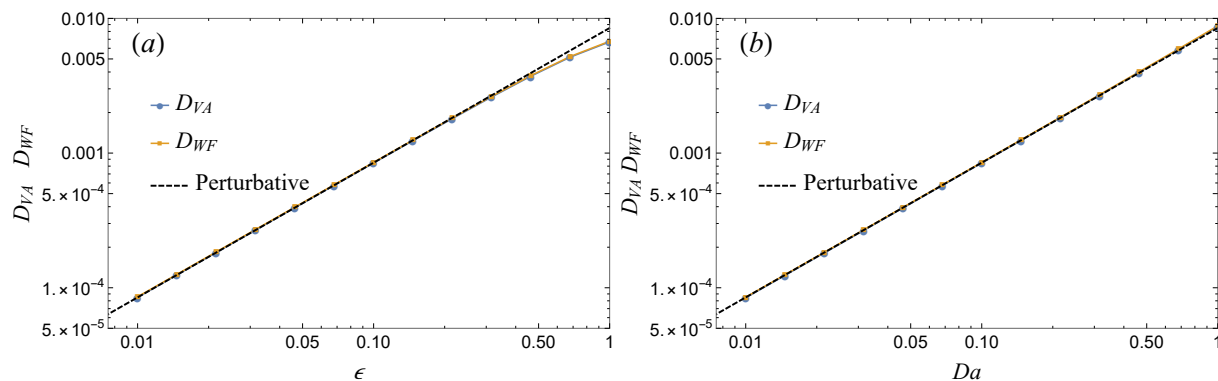
FIG. 2. Onsager cross coupling coefficients, D_{WF} and D_{VA} , computed using numerical simulations of the governing equations linearized around the equilibrium. In the panel (a) we fix Da = 0.1 and change \epsilon , while in panel (b) we fix \epsilon = 0.1 and we change Da . The remaining dimensionless numbers are \beta = 1 , \lambda = 1 and Pe = 1 .
