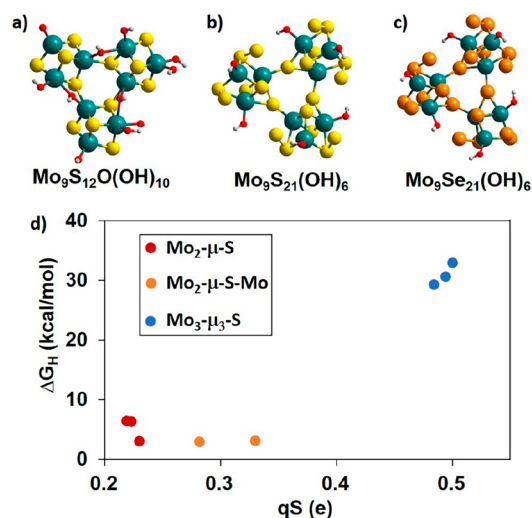
Figure 4. (a) \text{Mo}_9\text{S}_{12}\text{O}(\text{OH})_{10} , (b) \text{Mo}_9\text{S}_{21}(\text{OH})_6 , and (c) \text{Mo}_9\text{Se}_{21}(\text{OH})_6 trimers employed in DFT calculations. (d) Correlation between hydrogen adsorption free energy values \Delta G_{\text{H}} in kcal/mol and net atomic charge on the S atoms in \text{Mo}_9\text{S}_{21}(\text{OH})_6 trimers classified by type of S site.
