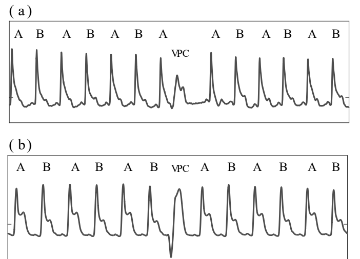
Fig. 1. Two TWA sequences including a VPC extracted from real ECG signals of patients undergoing a percutaneous transluminal coronary angiography (PTCA): in (a) the alternans sequence maintains the phase after the VPC while in (b) there is a phase shift after the VPC.
