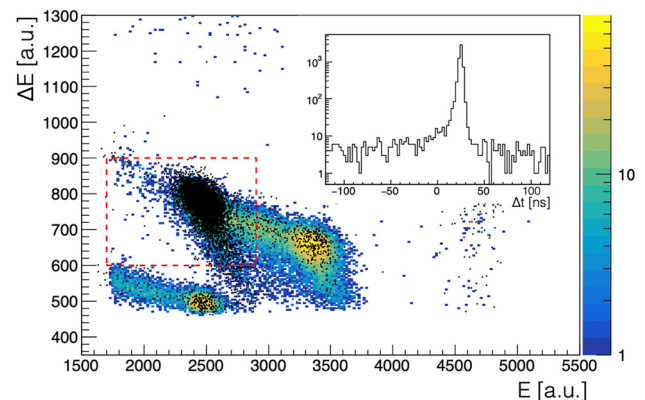
Fig. 3 \Delta E vs. E distribution obtained from the irradiation of a \text{CH}_2 target with a 28-MeV {}^7\text{Li} beam (color scale). The black dots are the events detected by the Si telescope in coincidence (within 200 ns) with an S1 signal in the TPC having a time profile compatible with a neutron-induced interaction. The dashed red box represents the {}^7\text{Be} selection cut used in the following analysis and described in Sect. 5.2. Inset: distribution of the time difference \Delta t between TPC and Si telescope for events within the 200 ns coincidence gate
