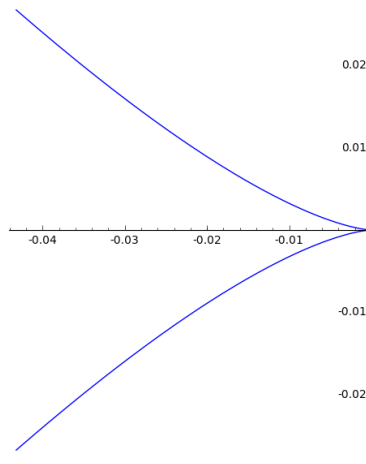
FIGURE 1. Example of a parametric plot (\Re \beta_2(\eta), \Im \beta_2(\eta))
