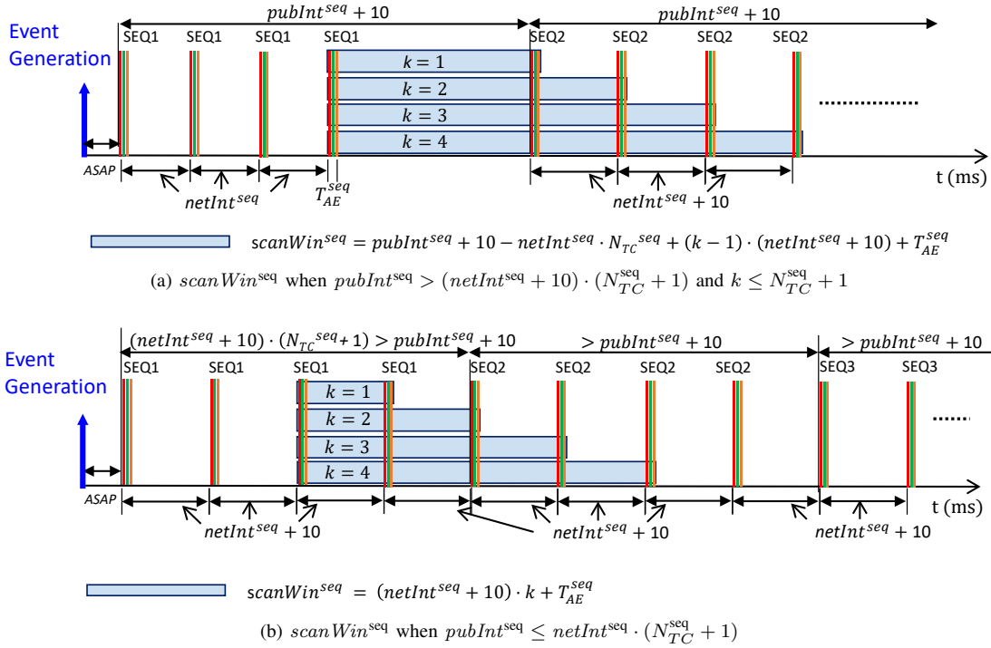
Fig. 6. Examples to calculate the optimum scanWin^{seq} .
