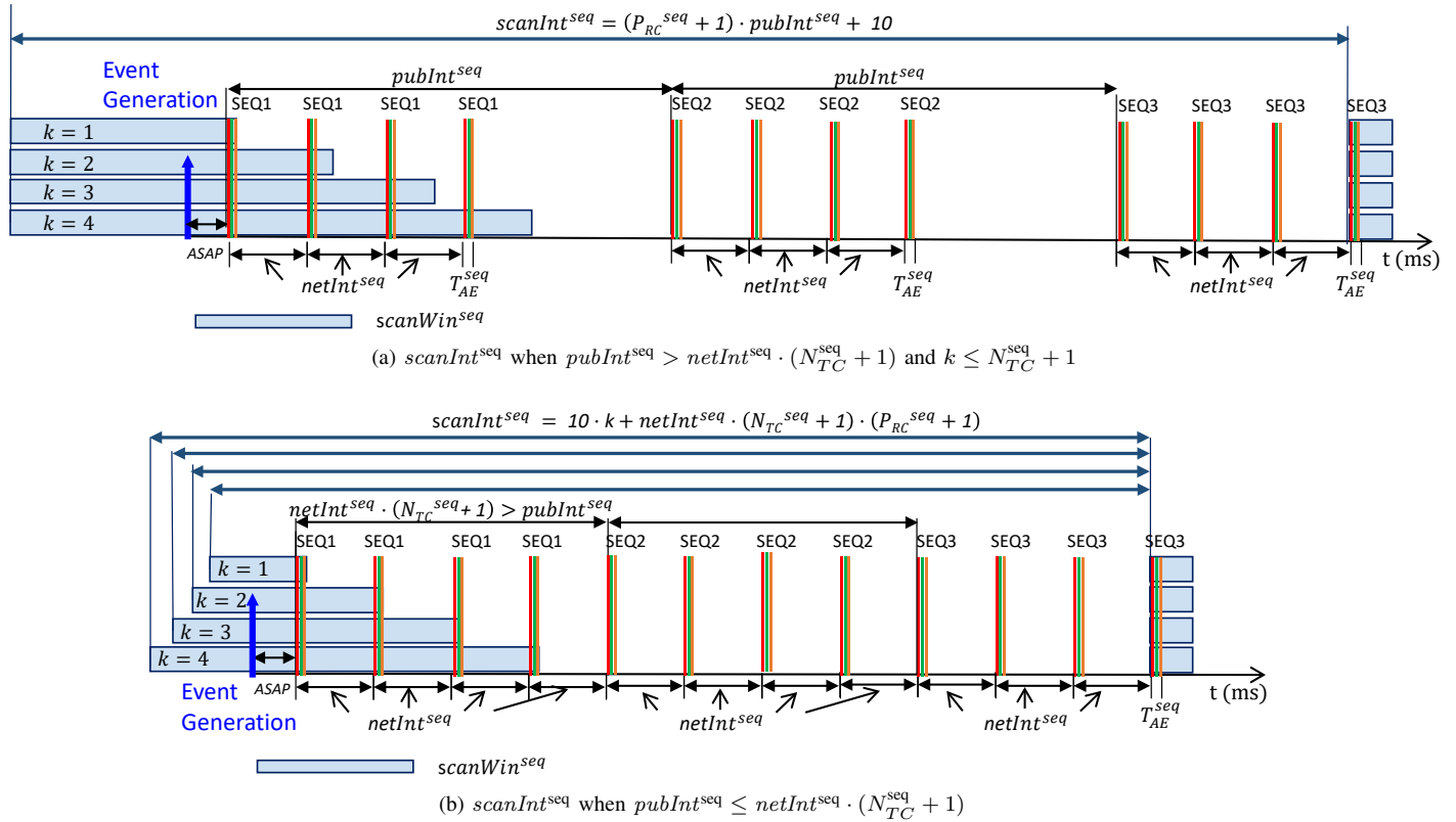
Fig. 7. Examples to calculate the optimum scanInt^{seq} .
