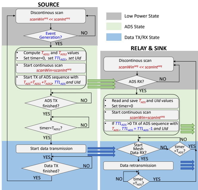
Fig. 5. BMADS algorithm.
