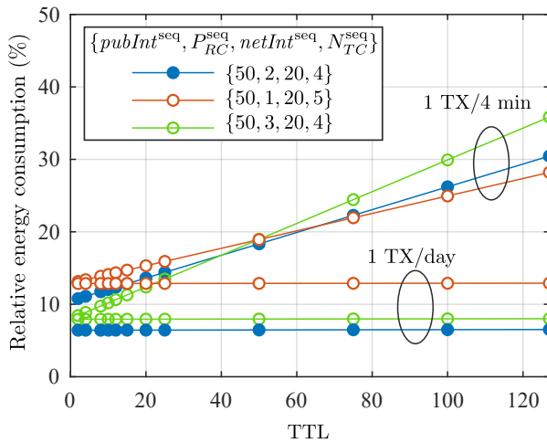
Fig. 13. Performance sensitivity to variations in the network size.
