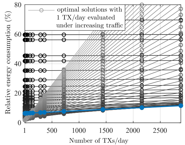
Fig. 11. Performance sensitivity to variations in traffic volume.
