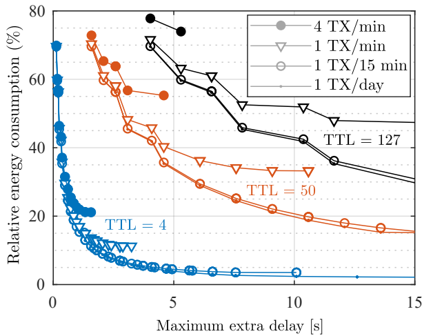
Fig. 10. Optimal solutions for different traffic volumes and network sizes.
