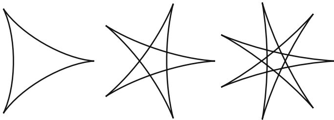
Fig. 5 Curves C_{k,k-1} for k = 2, 3, 4
