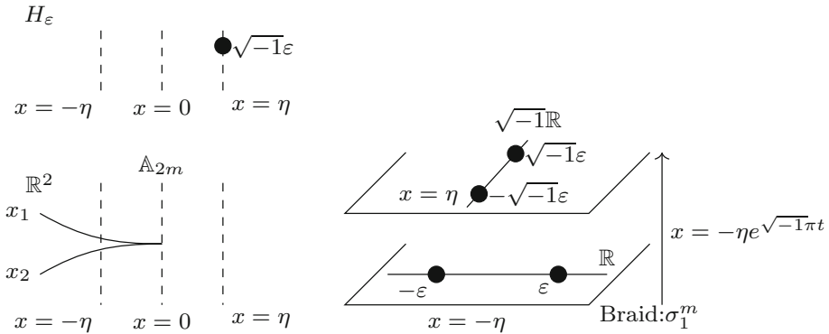
Fig. 7 Meridian at B_\varepsilon
