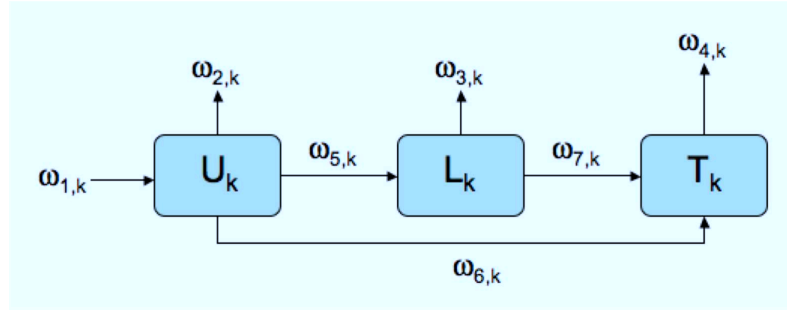
FIG. 1: Set of allowed transitions in the epidemic model within each connectivity class.
