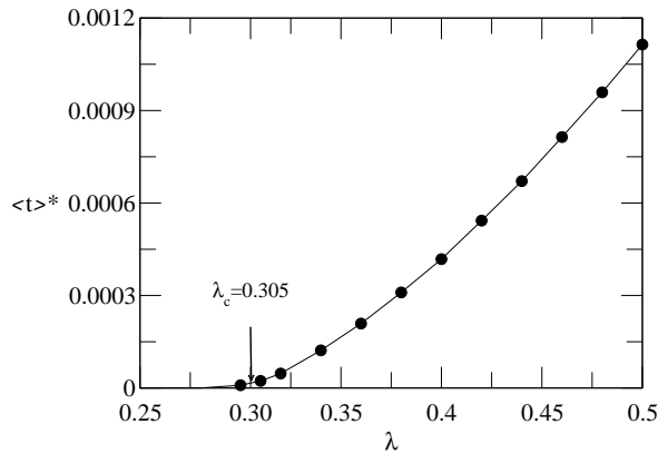
FIG. 2: Stationary proportion of sick individuals as a function of \lambda ( \in [0.25, 0.5] ) for p = 0.07 , r = 0.002 , \mu_{tb} = 0.2 , \mu = 0.009 and b = 0.01 . The arrow marks the position of the epidemic threshold ( \lambda_c = 0.305 ) as given by analytical calculations using the previous values for the parameters and the degree distribution. Error bars are smaller than symbol size. The initial size of the network, characterized by a degree distribution P(k, t_0) \sim k^{-3} , is N_0 = 10^6 . Each point is an average over at least 1000 values of \langle t \rangle^* .
