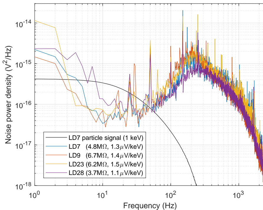
Figure 5. The noise power density spectra of the LD readouts compared with a signal of 1 keV in the frequency domain for one detector. This amplitude corresponds to a light signal associated to a full Q_{\beta\beta} energy release. To obtain the frequency representation of the signal, we take the square of the module of its Fourier transform, which has units V^2/Hz^2 . Then, we multiply it by the frequency bin in order to obtain the same units as the noise power density ( V^2/Hz ). The useful bandwidth is approximately 5–50 Hz. The low frequency noise spoils significantly the LD performance. Some peaks associated to vibrations are visible in the 10–50 Hz range. The Bessel cutoff frequency is 675 Hz. The computation of the sensitivities (in \mu V/keV ) given in the legend is explained in the text.
