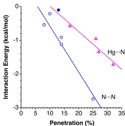
Fig. 4 Interaction energies between two molecules of [N_3-Hg(CF_3)] in dimeric topologies with torsion angles of 180^\circ ( 1a and 4a-7a , Scheme 3 and Table 1) as a function of the N \cdots N penetration indices at the energy minima (filled circle for 5a , empty circles for the rest), and estimated contribution (see text) of the Hg \cdots N contacts to the interaction energy in topologies with \tau = 90^\circ ( 1b , 2b , and 4b-7b ) as a function of the Hg \cdots N penetration index (triangles).
