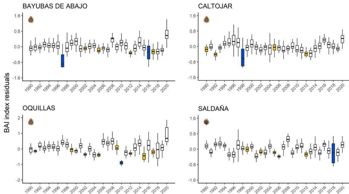
Fig. 3. Residuals of the climate growth model models over the period 1990–2020 for Bayubas ( P. nigra ; n=34 ), Caltojar ( P. nigra ; n=32 ), Oquillas ( P. nigra ; n=29 ) and Saldaña ( P. sylvestris ; n=37 ) stands. PPM and drought events are highlighted in blue and yellow, respectively. Boxplots vertical bars indicate the interquartile range.
