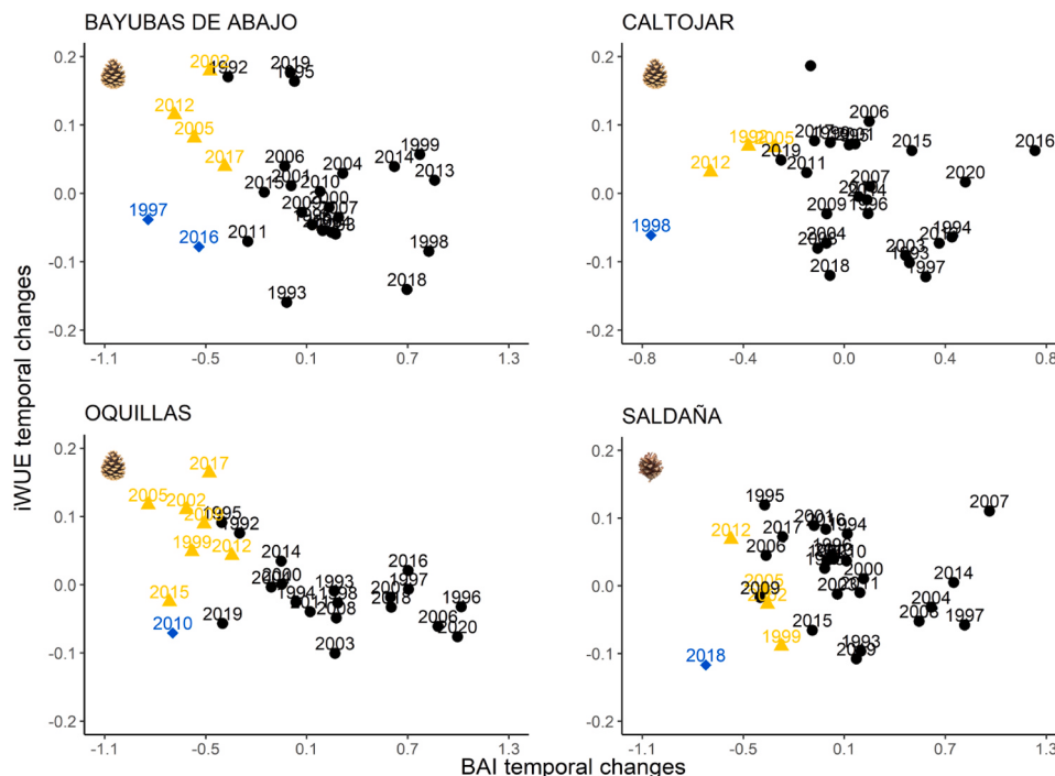
Fig. 4. Relationship between basal area increment (BAI) and intrinsic water-use efficiency (iWUE) temporal changes for Bayubas ( P. nigra ; n=5 ), Caltojar ( P. nigra ; n=5 ), Oquillas ( P. nigra ; n=5 ) and Saldaña stands ( P. sylvestris ; n=5 ) over the period 1990–2020. PPM and drought events are highlighted in blue and yellow, respectively.
