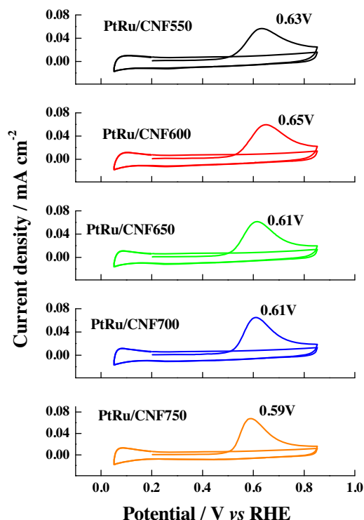
Fig. 5. (Colour online.) CO electrochemical oxidation on Pt–Ru catalysts supported on carbon nanofibers synthesized at different temperatures. Scan rate: 20 \text{ mV} \cdot \text{s}^{-1} . Supporting electrolyte: 0.5 \text{ M H}_2\text{SO}_4 . CO adsorption potential: 0.2 \text{ V} vs. RHE.
