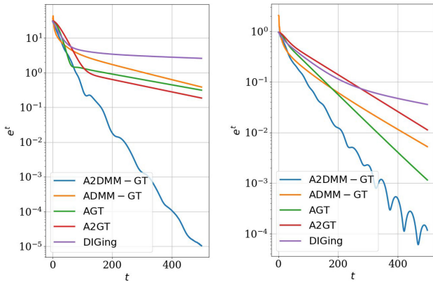
Fig. 2. Evolution of the error with time for the five protocols under comparison. Left is the quadratic programming setup, right is the linear classification setup.
