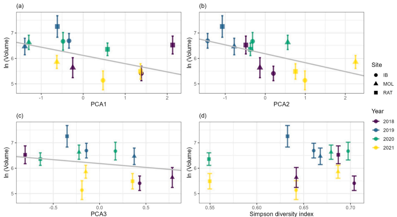
Fig. 3. Relationships between volumes of the hypervolumes and the habitat conditions. Relationships between volumes (means of \ln -transformed values \pm SDs) of the 12 hypervolumes calculated for aquatic plant communities through space and time and the three principal component (PCA) axes describing abiotic conditions (a–c) and the Simpson diversity index (d). Volumes indicate hypervolume sizes based on the five traits considered, and reflect the variability of community-level growth strategy. Gray lines reflect significant effects ( p < 0.01 ) of explanatory variables in fitted linear mixed-effects models. PCA1, trophic status; PCA2, thermal conditions; PCA3, pH and dissolved oxygen concentration. SD, standard deviation.
