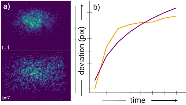
Fig. 5. We have analyzed that bias in the datasets used in this work [12] and found that this behavior diminishes over time. (a) Distribution of scanpath fixations in two different time instants for the whole training dataset. (b) We have computed the standard deviations of fixations (y-axis) over time (x-axis) for all the ground-truth scanpaths (in orange) and found they increase in a logarithmic fashion (the fitted curve is shown in purple).
