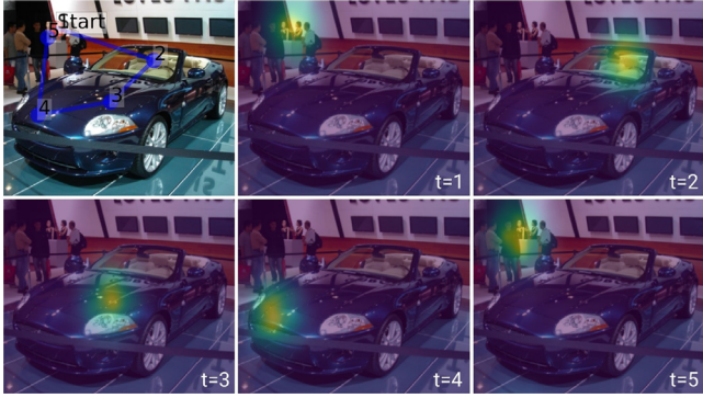
Fig. 3. An example of our spatialized scanpath representation. The top left image shows a RGB image with a sample ground-truth scanpath overlaid. For that sample ground-truth scanpath, we transform each fixation point into a Gaussian map centered at that particular point (see Section 3.1).
