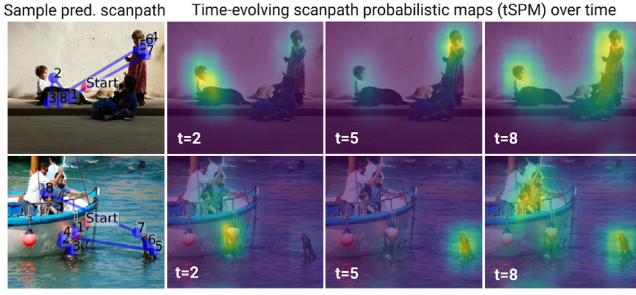
Fig. 4. We show, for two given test images, the evolution of our predicted time-evolving scanpath probabilistic maps (tSPM, see Section 3.2) over time. Our Bayesian approach enables a probabilistic weight selection for the next fixation, and allows our model to be stochastic, while the ConvLSTM module allows taking into account the previous fixations (see Section 3.4).
