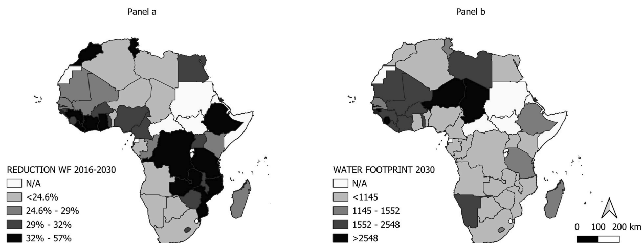
Fig. 4. Reduction of the WF (%) in the period 2016–2030 driven by changes in per capita GDP (panel a) and projected average crop WF ( \text{m}^3/\text{ton} ) in 2030 (panel b).
