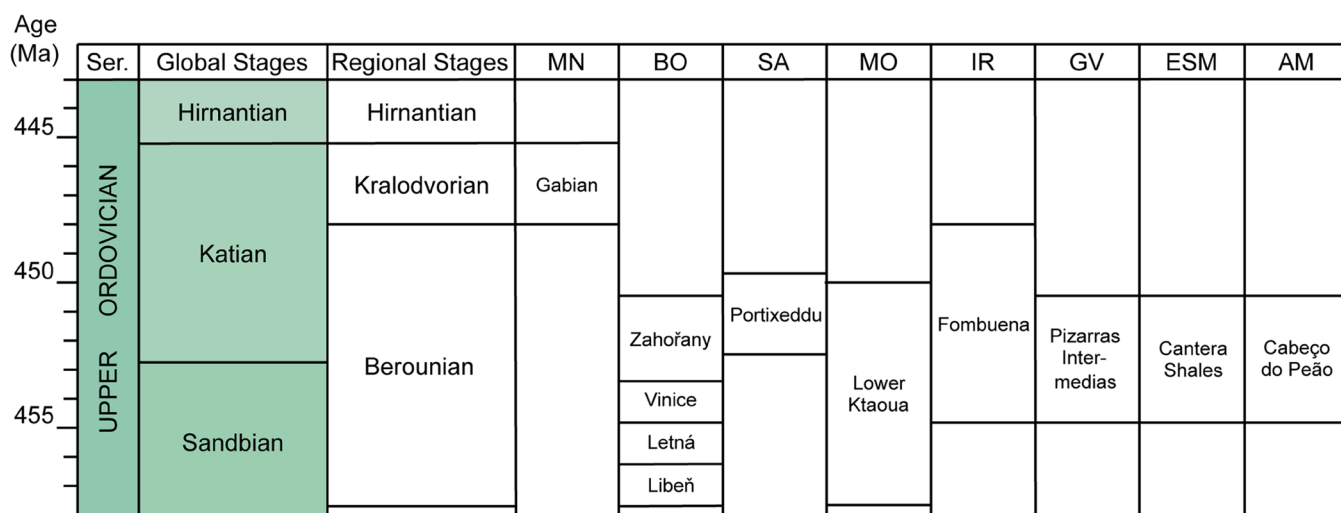
Figure 2. Stratigraphic correlation of formations in which Rhombifera occurs. MN , Montagne Noire, France; BO , Bohemia; SA , Sardinia; MO , Morocco; IR , Iberian Ranges, Spain; GV , Guadarranque – Villuercas, Spain; ESM , Eastern Sierra Morena, Spain; AM , Amêndoa – Mação, South of the Central Iberian Zone, Portugal; Ma , million years before present; Ser. , series.
