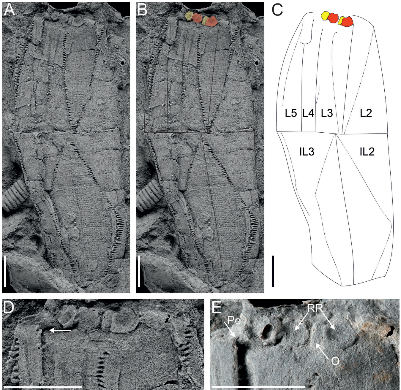
Figure 5. Latexes of the lectotype of Rhombifera bohémica Barrande, 1867, NMP L13001. A , Lateral view showing the infralateral plates (below), lateral plates (above) plus two orals and two radials (top). Note the very large IL:IL pectinirhomb (below) and asymmetrical L:L pectinirhomb above; B , the same with outlines of the thecal plates indicated; C , interpretation of the visible thecal plating. Radial plates red, orals yellow; D , detail of the top of the theca showing notch for periproct in plate L5 (arrowed); E , slightly different view of top of theca with radial and oral plates indicated. Latexes whitened with ammonium chloride. IL2 , IL3 Infralateral plates, L2–L5 Lateral plates, O oral plate, Pe notch for periproct, RR radial plates; scale bars = 5 mm.
