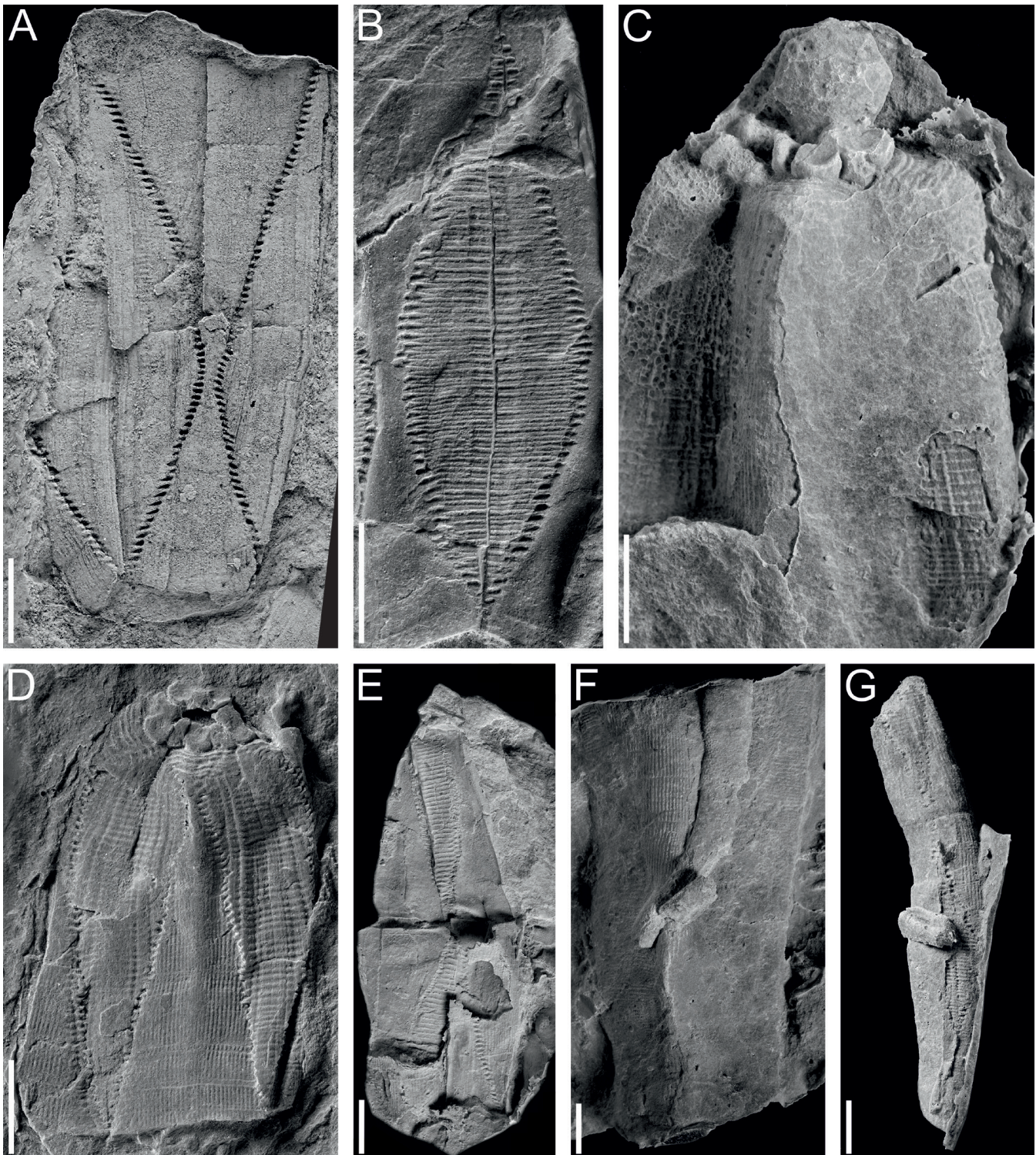
Figure 4. Latexes of Rhombifera bohemica Barrande, 1867, from the Czech Republic (A, B, D–F) and Spain (C, G). A, Paralectotype NMP L13000. External surface of large IL:IL pectinirhomb. Note short slits; B, SU.PAL.2017.054.15 Internal surface of IL:IL pectinirhomb. Note traces of dichopores between pectinirhomb slits; C, lateral view of MPZ 2023/91 showing large lateral plates plus some orals and radials (top). Note the lobate outline of the theca; D, 'Kesling's specimen' SU.PAL.2017.054.16 showing complete oral and radial circlet. Note the external ornament; E, UCBL-EM 12149. Another example showing both the IL and L circlets with two aligned rhombs; F, MPZ 2023/94, Huerva Member, Fombuena Formation, Santa Catalina (Fombuena), Spain. External surface of a large infralateral plate showing fine vertical growth lines between the rhombs (centre top) and similar horizontal traces of the dichopores within the rhombs (top right); G, lateral view of specimen MPZ 2023/90 showing infralateral and lateral circlets. Latexes whitened with ammonium chloride; scale bars = 5 mm.
