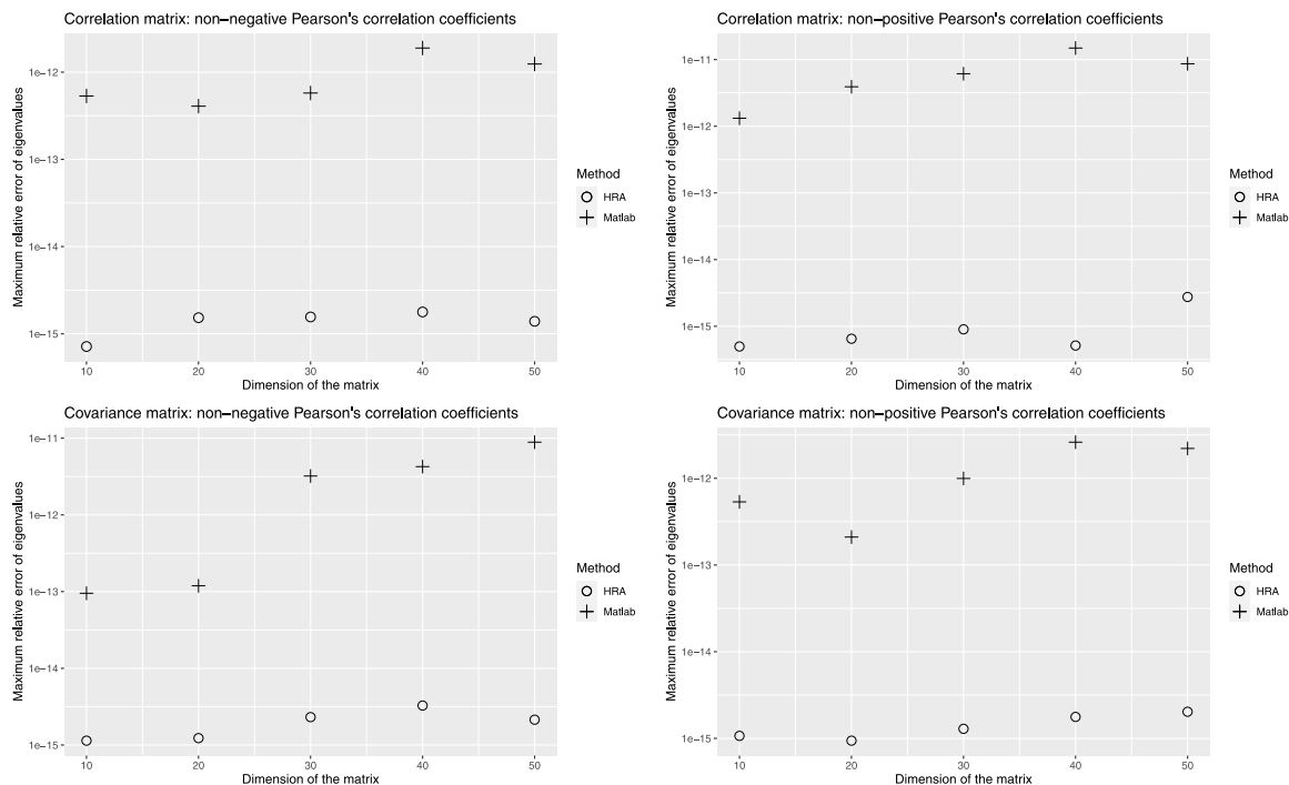
Fig. 1. Maximum relative error in the computation of the eigenvalues by the function eig from Matlab and the TNEigenValues routine for matrices of different dimension.
