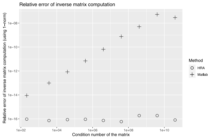
Fig. 3. Relative error in the computation of the inverse matrix by the function inv from Matlab and the TNInverseExpand routine for matrices of different condition number.
