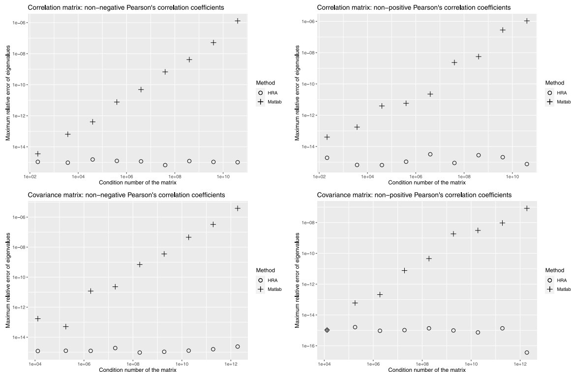
Fig. 2. Maximum relative error in the computation of the eigenvalues by the function eig from Matlab and the TNEigenValues routine for matrices of different condition number.
