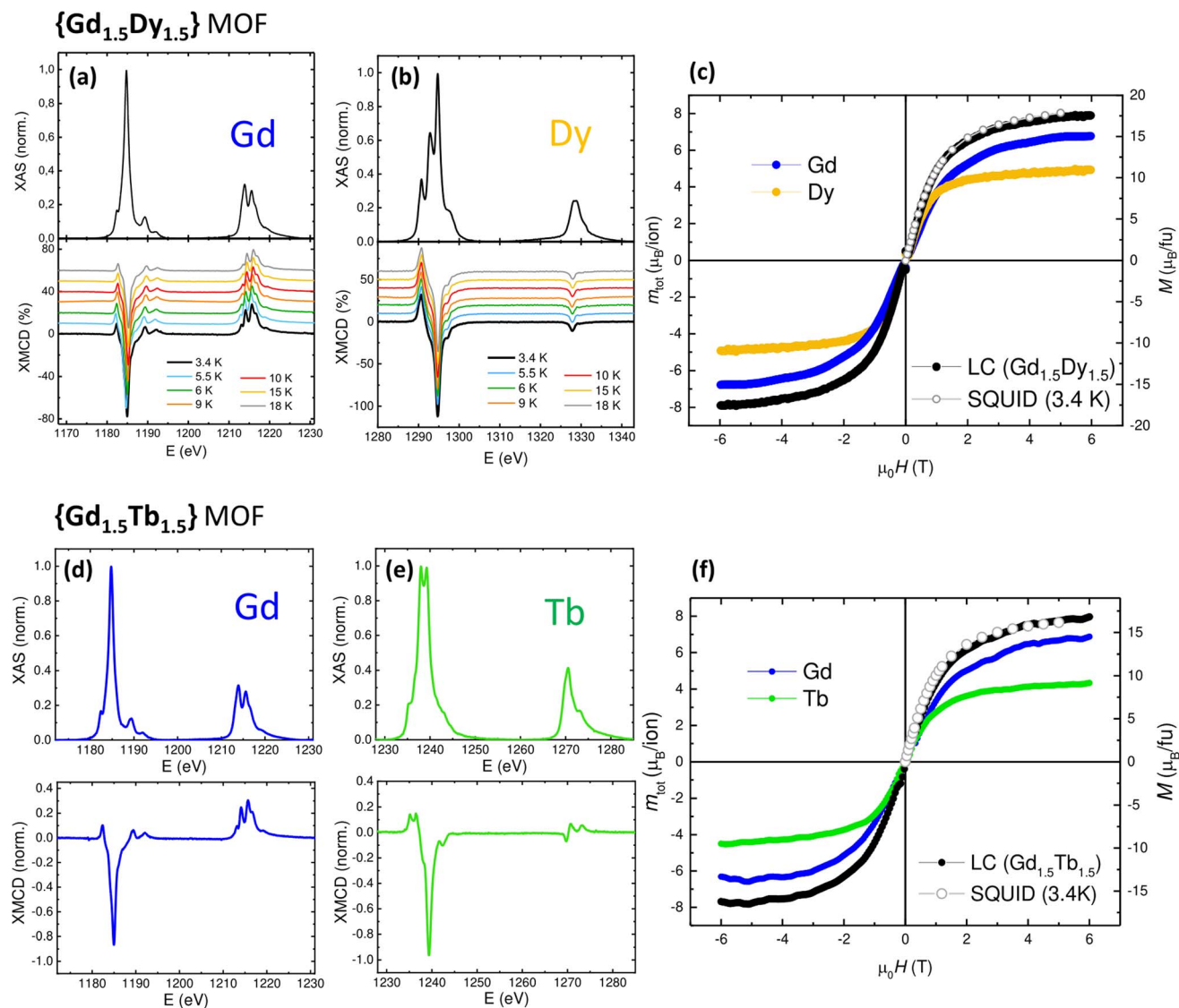
Fig. 3 XAS and XMCD characterization. Gd_{1.5}Dy_{1.5} : normalized, background-subtracted XAS (top) and XMCD (bottom) spectra measured across the M_{4,5} edge of Gd (a) and Dy (b) at 6 T and indicated temperatures, between 3.4 K and 18 K; (c) field-dependence of the total magnetic moment, m_{TOT}(H)/ion , obtained for Gd^{3+} and Dy^{3+} , and magnetic moment per formula unit, at 3.4 K. Open symbols show, for comparison, the magnetization curve M(H) of the mixed MOF determined by SQUID at the same temperature; Gd_{1.5}Tb_{1.5} : XAS and XMCD (6 T and 3.4 K) across the M_{4,5} edges of Gd (d) and Tb (e); (f) m_{TOT}(H)/ion obtained for Gd^{3+} and Tb^{3+} , calculated magnetic moment per formula unit at 3.4 K (black filled symbols), and SQUID determined M(H) (open symbols).
