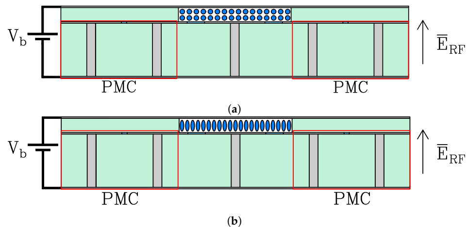
Figure 1. Polarization of the LC in the nematic state: (a) V_b < V_{th} , (b) V_b \geq V_{sat} .
