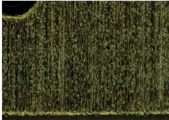
Figure 8. MRGW-LC resonator's microscope image with microgrooves.
