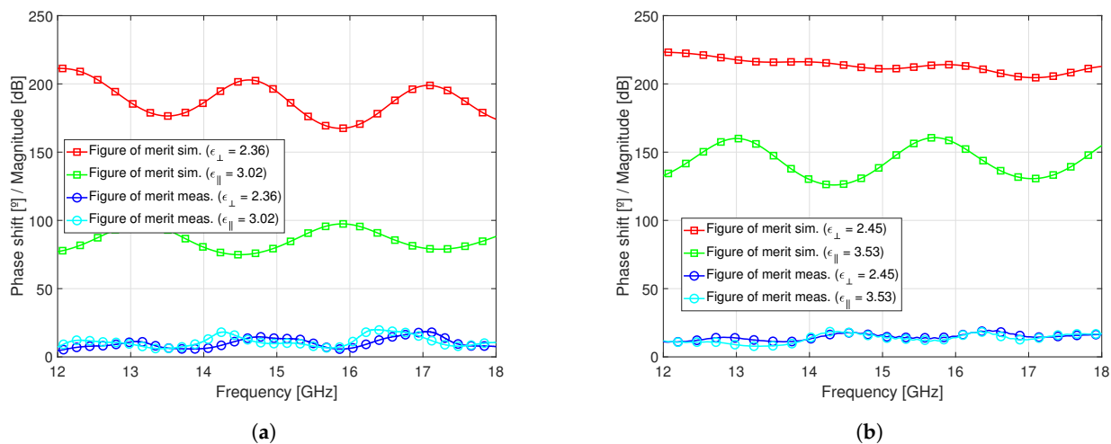
Figure 15. Figure of merit comparison between the simulated and measured responses of the phase shifter filled with (a) GT3-23002 and (b) GT7-29001.
