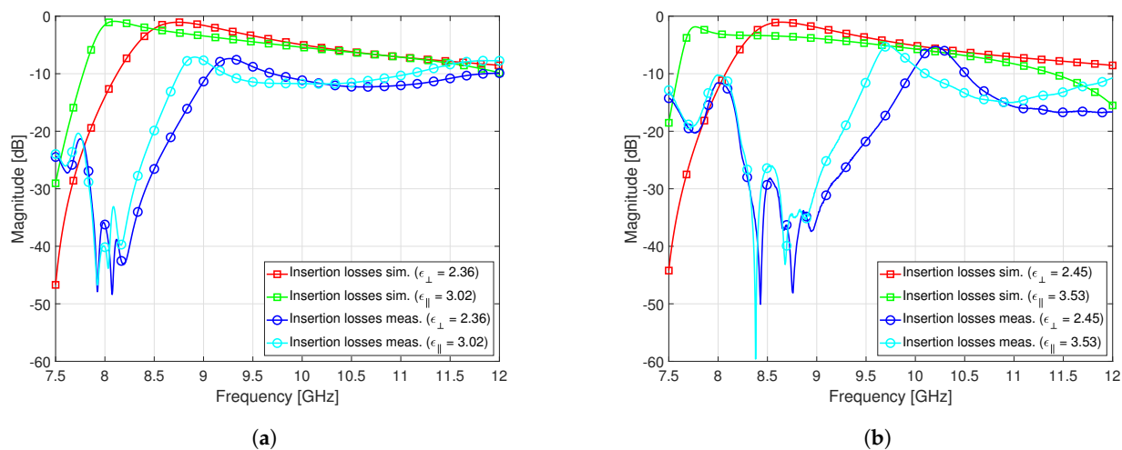
Figure 12. Comparison of the frequency responses of the simulated and measured responses of the resonator filled with (a) GT3-23002 and (b) GT7-29001.
