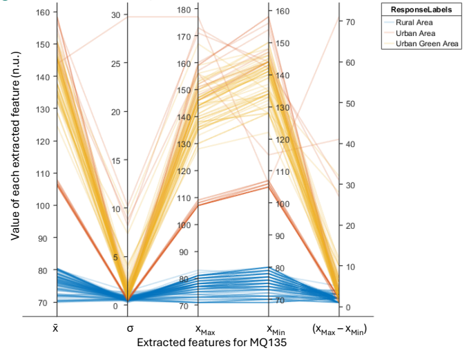
Fig. 7 Extracted features from MQ135.
