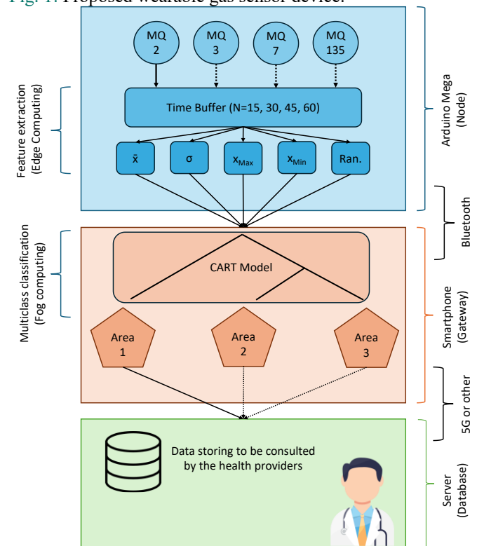
Fig. 2: Proposed wearable gas sensor device.
