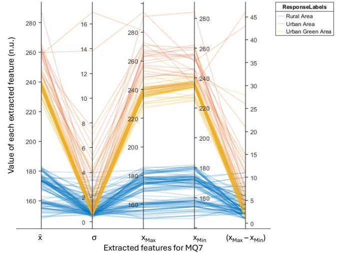
Fig. 6 Extracted features from MQ7.
