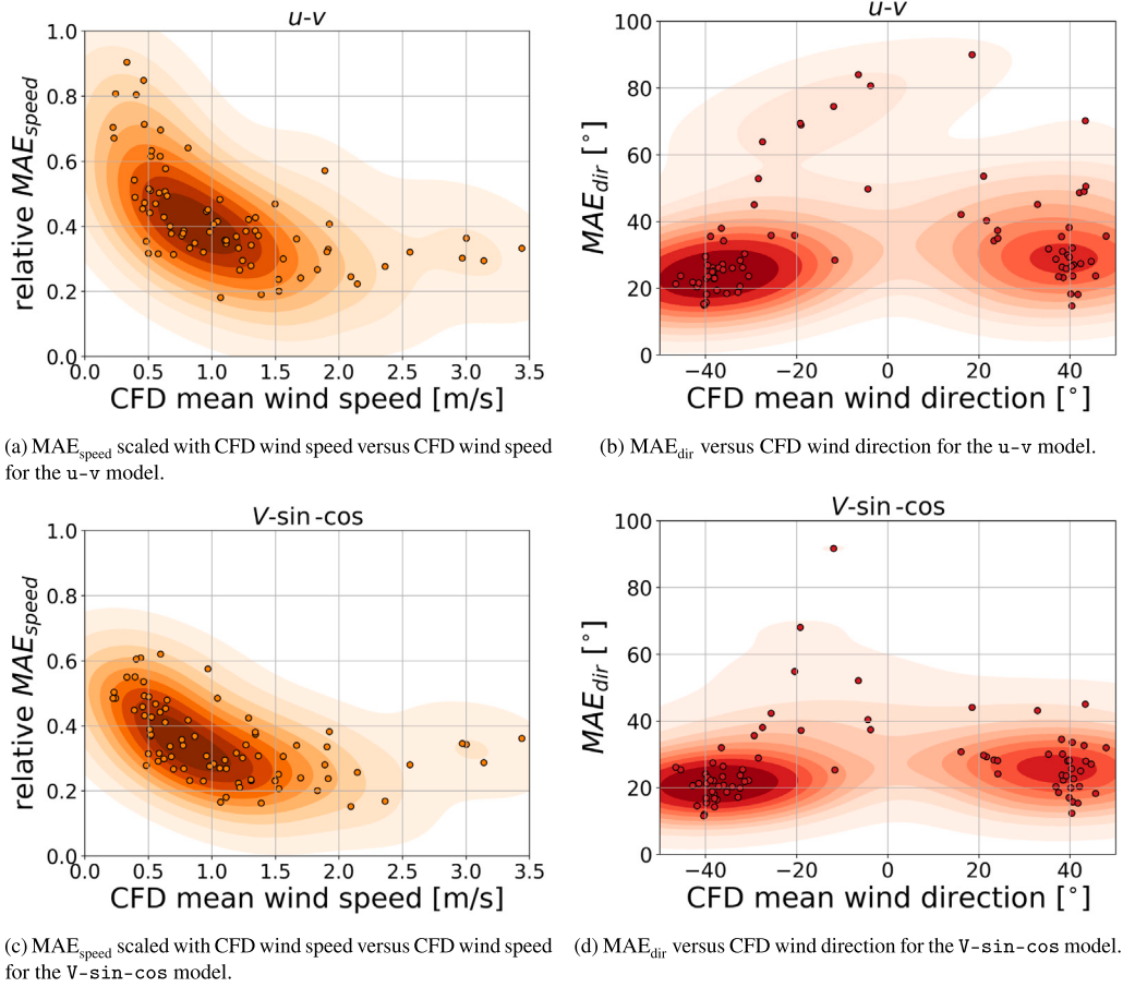
Fig. 6. Relative MAE_{speed} and MAE_{dir} versus CFD wind speed and direction averaged for each of the 80 test events for 128 \times 128 resolution u-v model and V-sin-cos model. Relative MAE_{speed} is MAE_{speed} divided by the mean CFD wind speed of the event.
